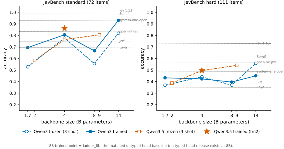
Figure 3: JevBench (public subset) standard and hard accuracy against backbone size. Qwen3 trained (solid; each point uses the recipe named for its row in Table 2) and frozen with three exemplars (dashed); Qwen3.5 frozen controls at 2B/4B/9B and the trained Qwen3.5-4B (star). Dotted lines mark other public entries on the same ids, whose rendering and protocols differ (Appendix A.13). Intervals are in Table 2.
