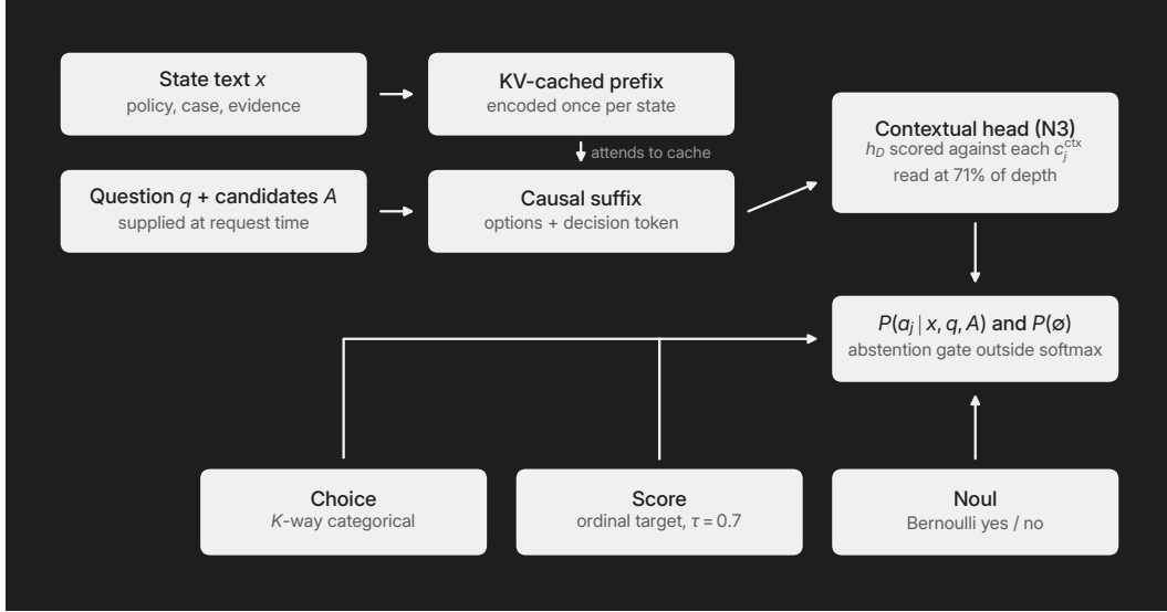
Figure 1: The decision pass. The state is encoded once into a key-value cache. Each question is a short causal suffix holding the question and its runtime candidates; the head reads the terminal decision state h_D against each candidate’s pooled contextual state c_j^{\text{ctx}} at 71% of backbone depth. One readout serves three typed contracts (Choice, Score, Noul), and abstention is a separate gate outside the candidate softmax.
