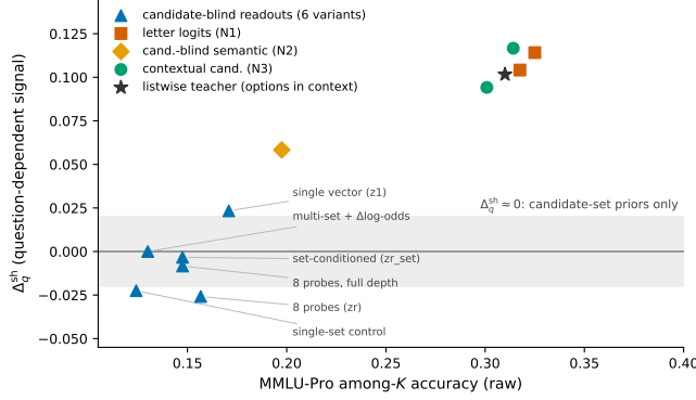
Figure 2: Raw MMLU-Pro among- K accuracy against \Delta_q^{\text{sh}} ( n=1,200 ; shaded: the \pm.02 band of Section 5.3). The six candidate-blind variants cluster at zero at every head capacity, objective and depth; the letter-logit (N1) and contextual (N3) readouts and the listwise teacher carry .09–.12, and the semantic readout N2 sits between. Accuracy alone does not separate the groups.
