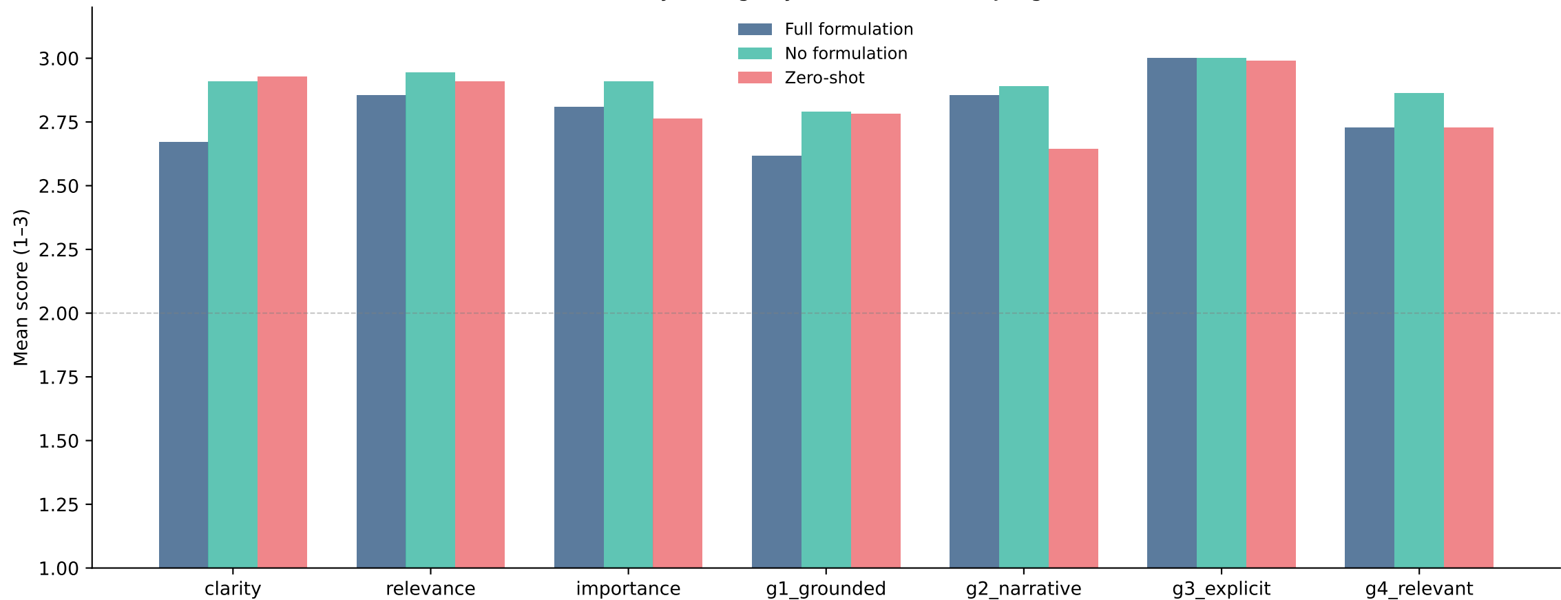
Quality Ratings by Condition — LLM Judge
