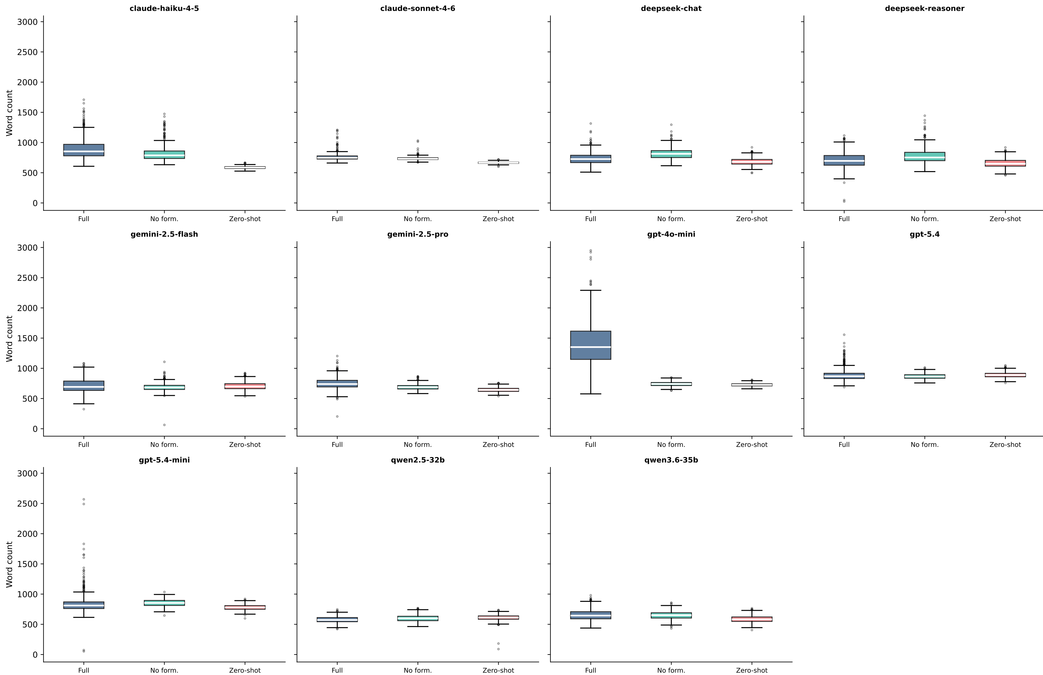
Word Count Distribution per Model × Condition
