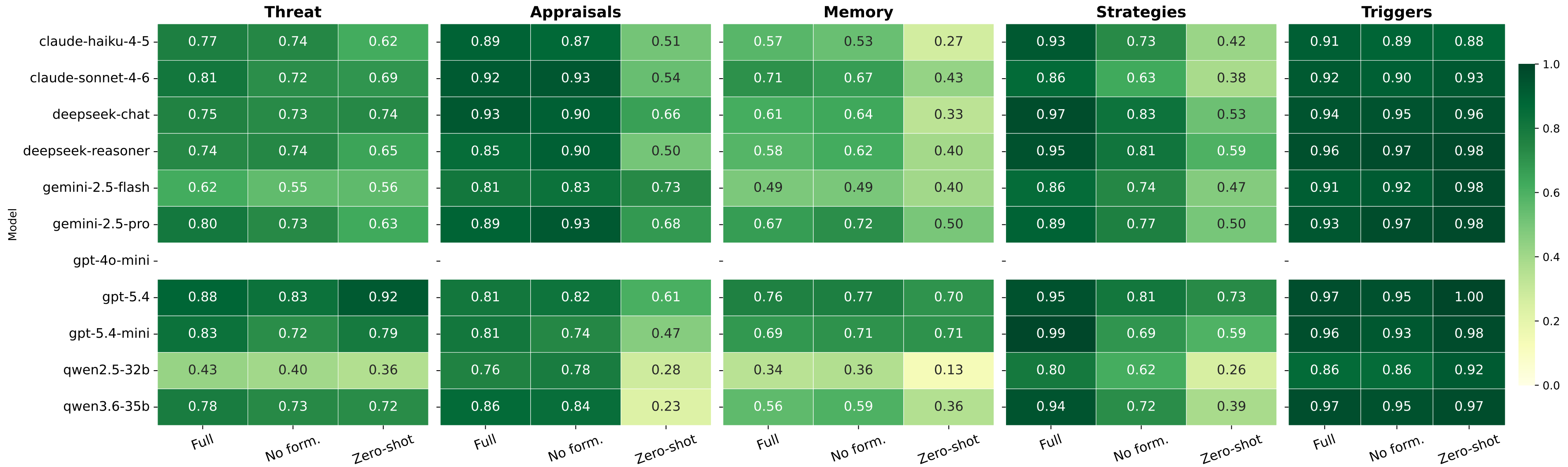
DeepSeek-v4-flash — E&C coverage per model × condition
