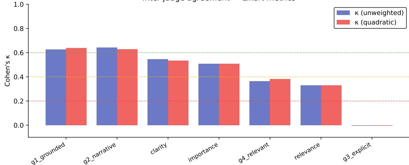
Inter-judge agreement — Likert metrics
