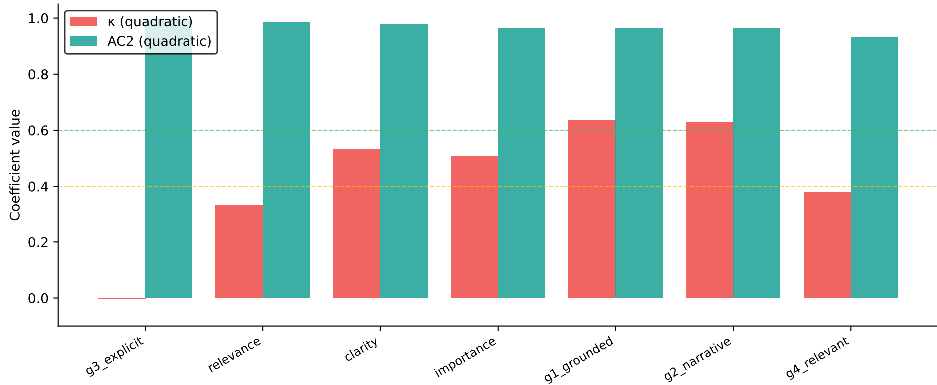
Inter-judge agreement — weighted \kappa vs AC2 on Likert metrics
