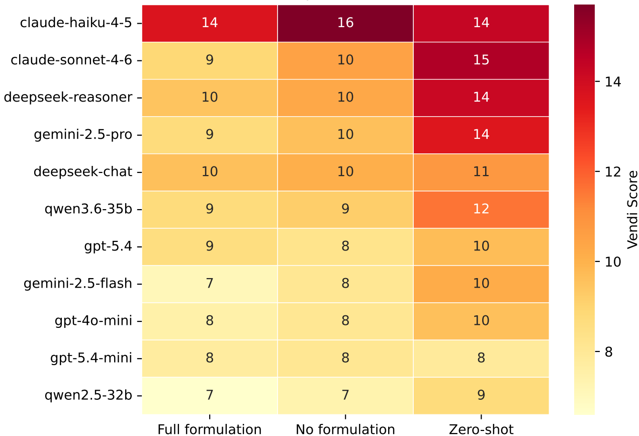
Vendi Score per model × condition
