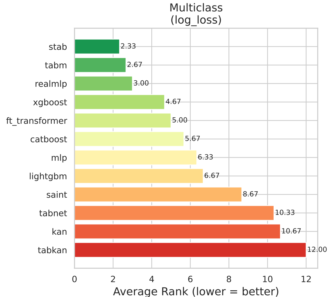
Average Rank per Task Type (Rank 1 = Best)
