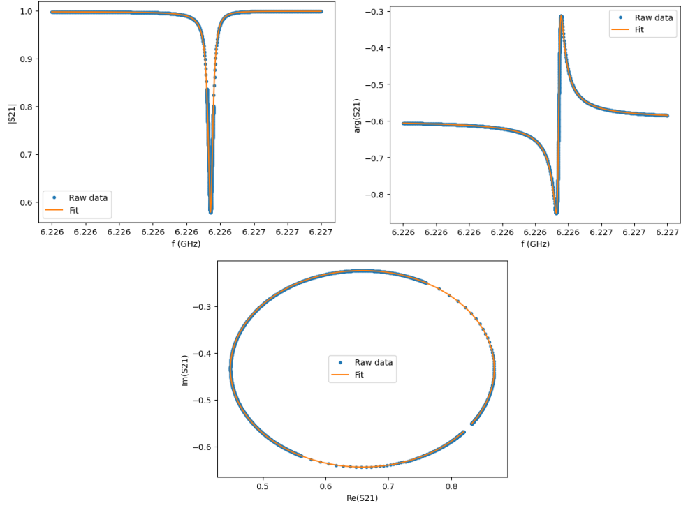
Figure 15: Fittings following [5] used to extract the quality factor from the simulated S_{21} spectrum of the 4H-SiC resonator with f_r = 6.22 GHz
