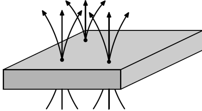
Figure 4: Schematics of the penetration of magnetic flux lines through a Type-II superconductor. Reproduced from [4].
