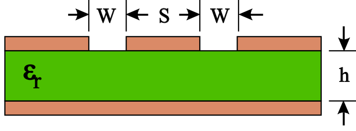
Figure 7: Physical parameters required for calculations using conformal mapping in Eqs. (2.8) and (2.9). Reproduced from [13].
