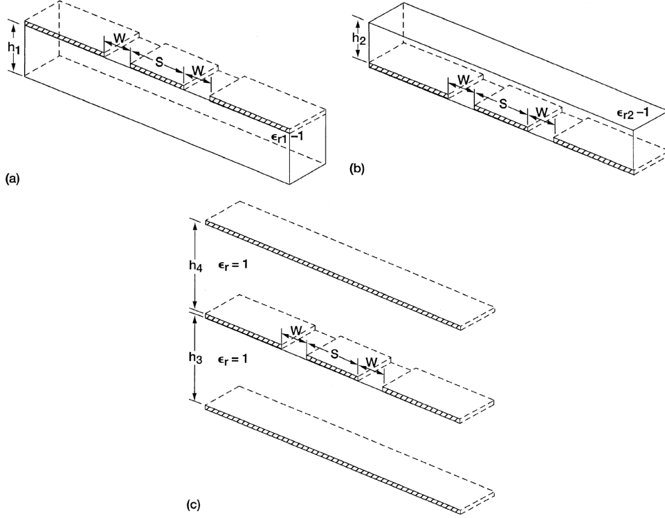
Figure 6: Schematics of the three different partial capacitances calculated using conformal mapping techniques for a coplanar waveguide sandwiched between two dielectric volumes. Reproduced from [8].
