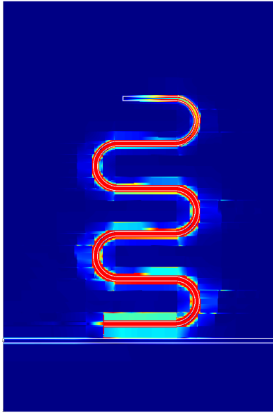
(c) 6H-SiC, in resonance
