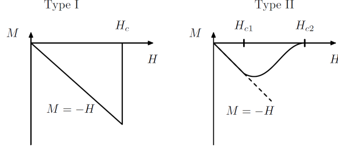
Figure 3: Visual representation of the abrupt transition of the internal flux, presented by a Type-I superconductor, in comparison with the smooth transition presented by a Type-II superconductor. Reproduced from [4].
