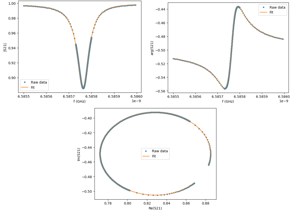
Figure 17: Fittings following [4] used to extract the quality factor from the simulated S_{21} spectrum of the diamond resonator with f_r = 6.59 GHz
