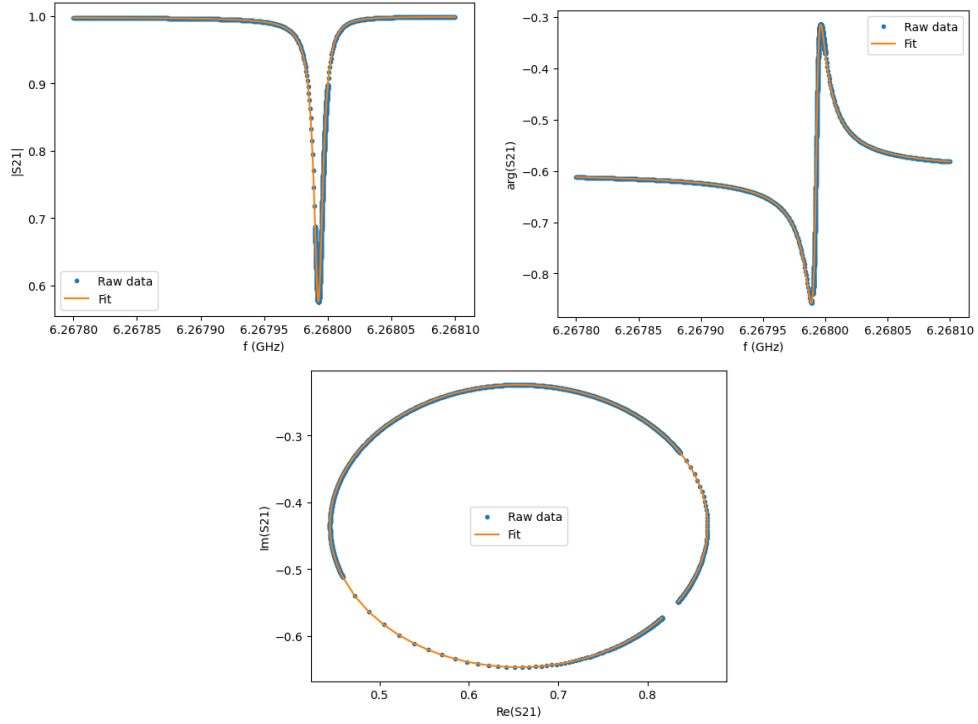
Figure 16: Fittings following [4] used to extract the quality factor from the simulated S_{21} spectrum of the 6H-SiC resonator with f_r = 6.27 GHz
