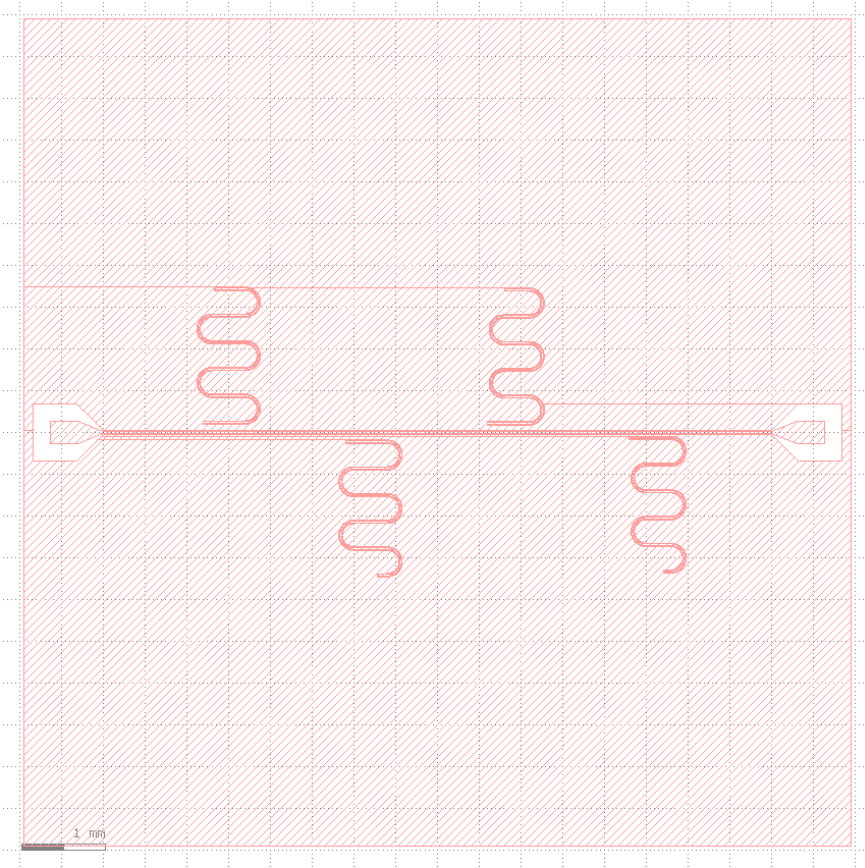
(a) 6H-SiC positive layout
