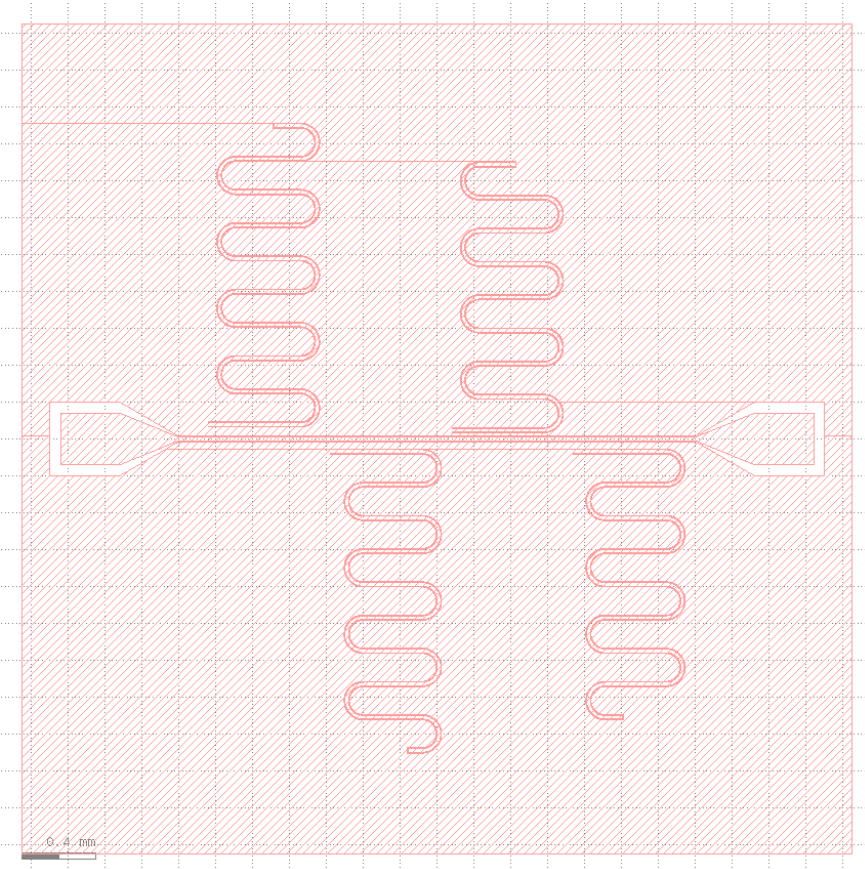
(b) Diamond positive layout
