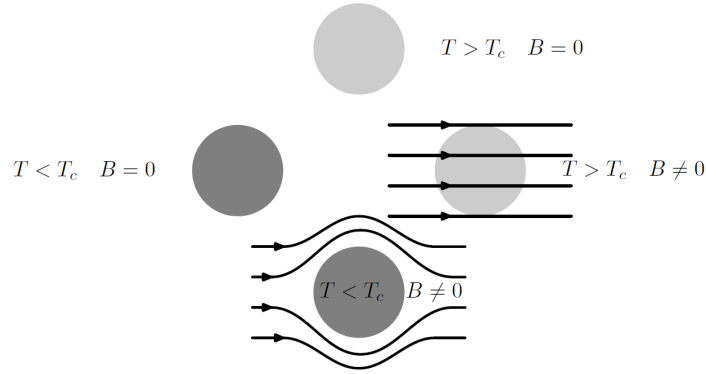
Figure 2: Meissner Ochsenfeld effect representation. Reproduced from [3]
