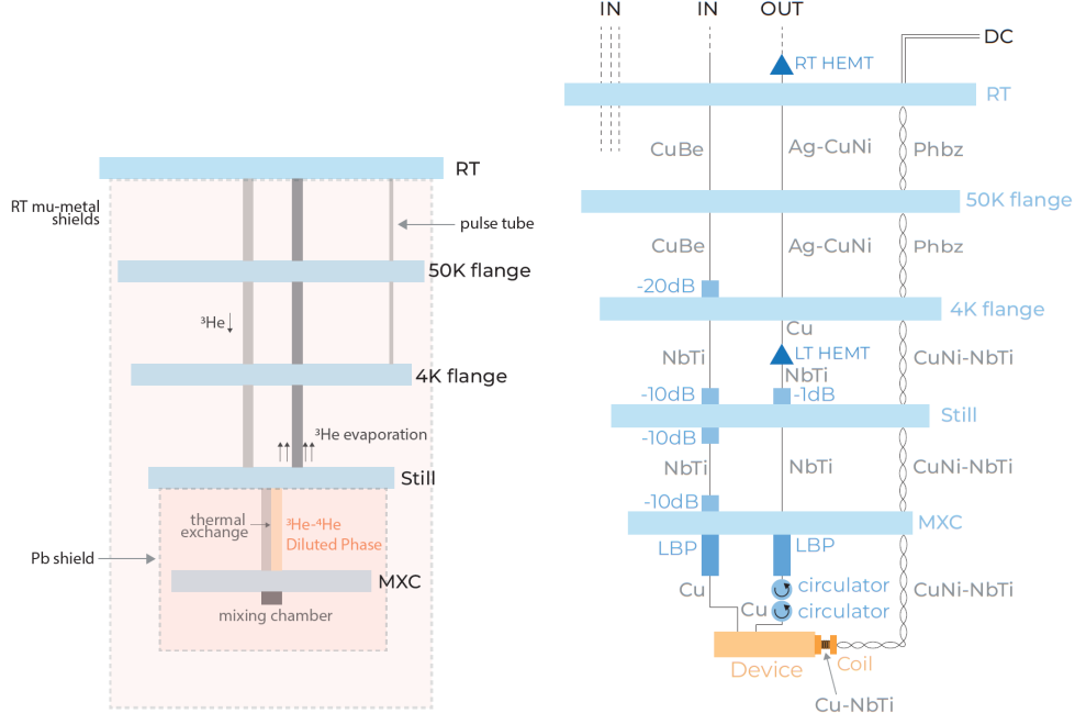
Figure 9: Reproduced from [16]. Cryogenics schematics of Bluefors fridge, analogous to Leiden fridge setup. Circuitry schematics of Bluefors fridge, analogous to Leiden fridge setup.
