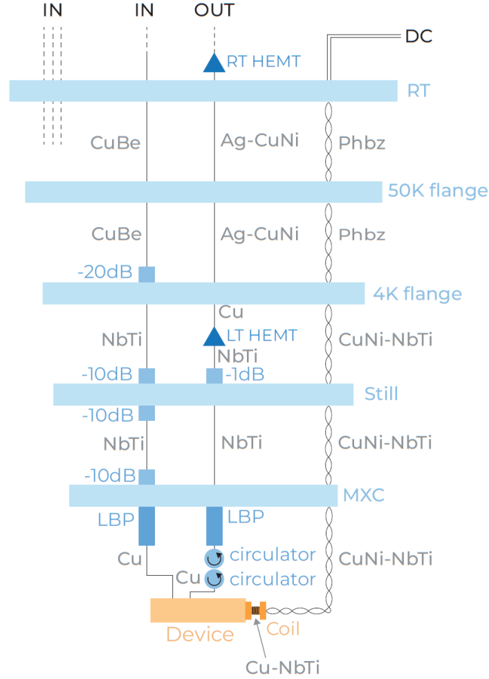
Figure 10: Reproduced from [16]. Circuitry schematics of Bluefors fridge, analogous to Leiden fridge setup.
