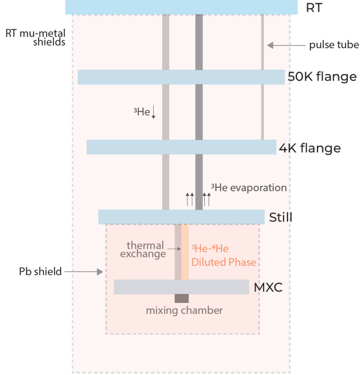
Figure 9: Reproduced from [16]. Cryogenics schematics of Bluefors fridge, analogous to Leiden fridge setup.
