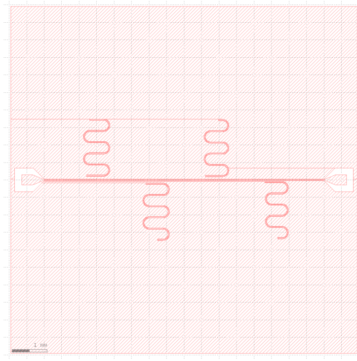
Figure 10: Positive layout used for the wet etching process.
