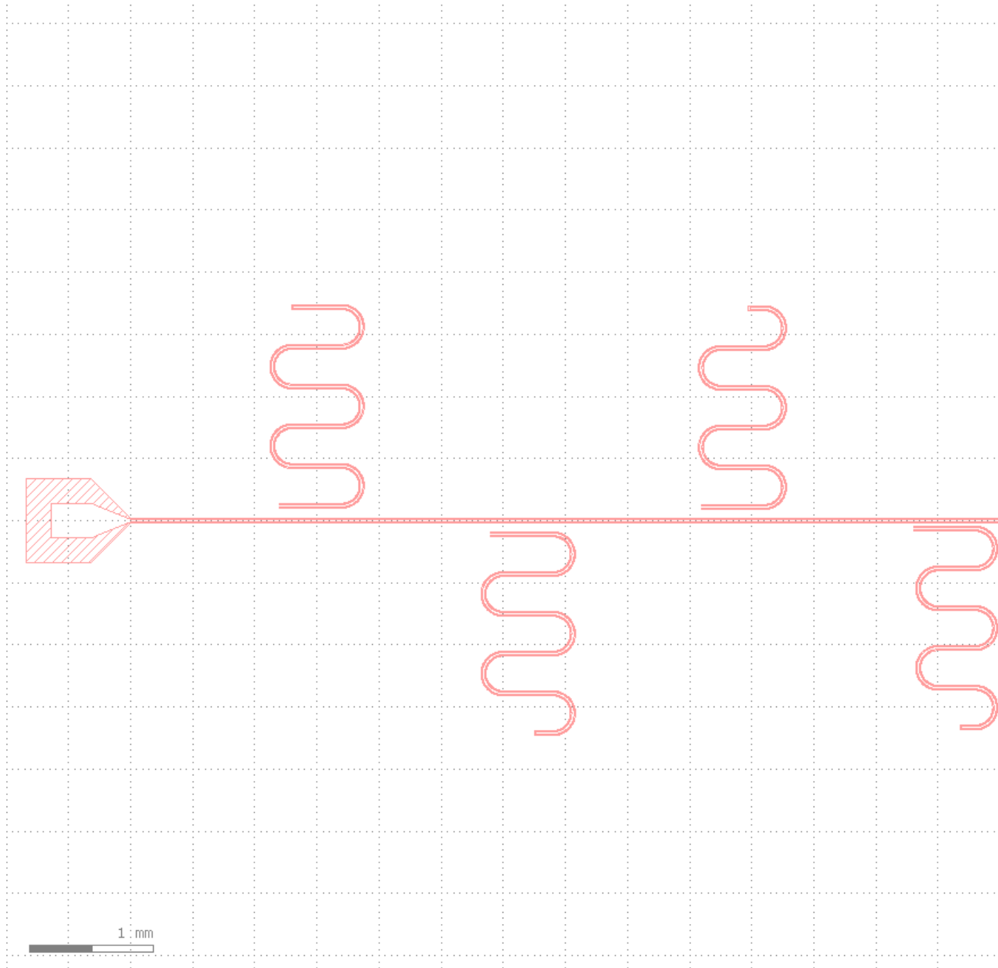
Figure 11: Negative layout used for the lift-off process.
