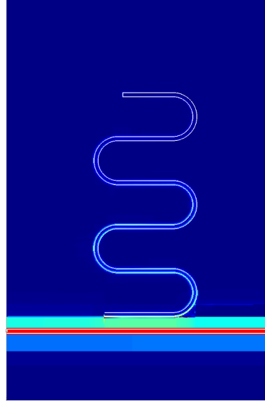
(b) 6H-SiC, out of resonance
