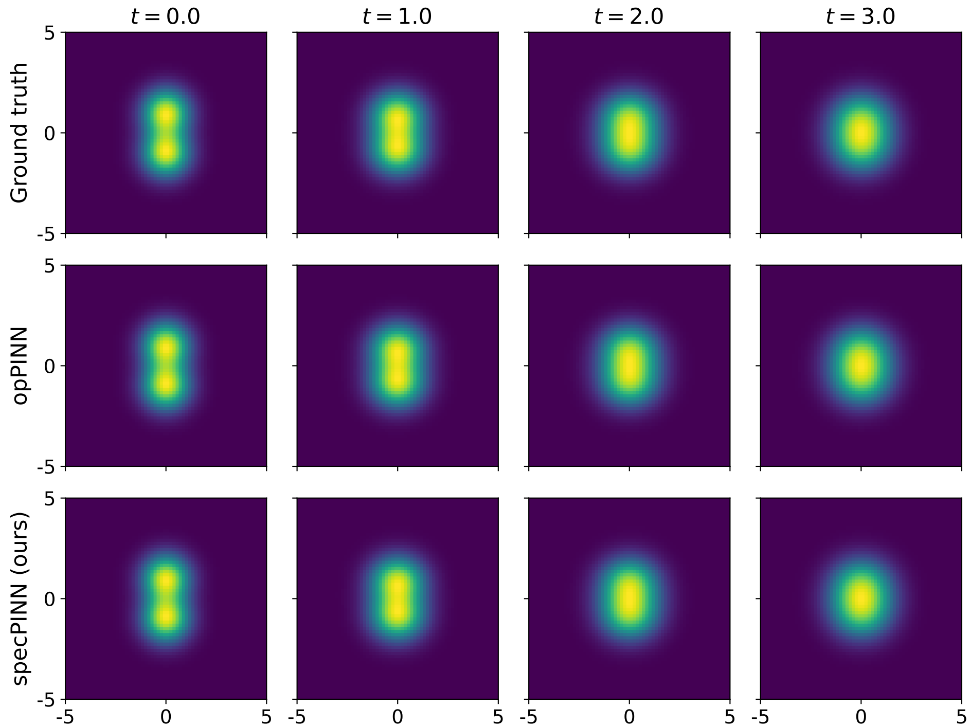
Initial condition (5.1) ( \gamma = 0 , \Lambda = 5/16 )
