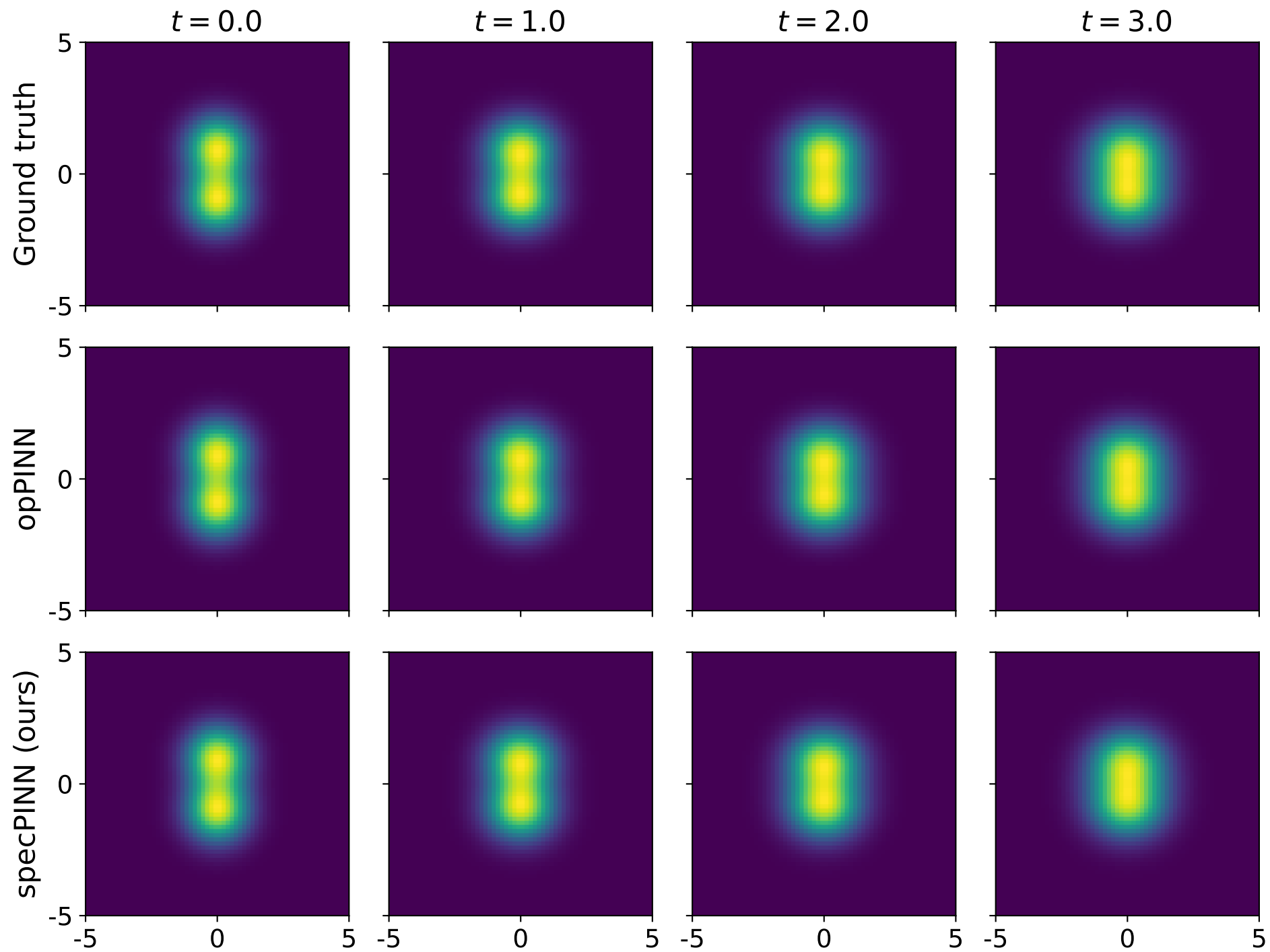
Sum of two Maxwellian distributions ( \gamma = 1.00 , \Lambda = 0.06 )
