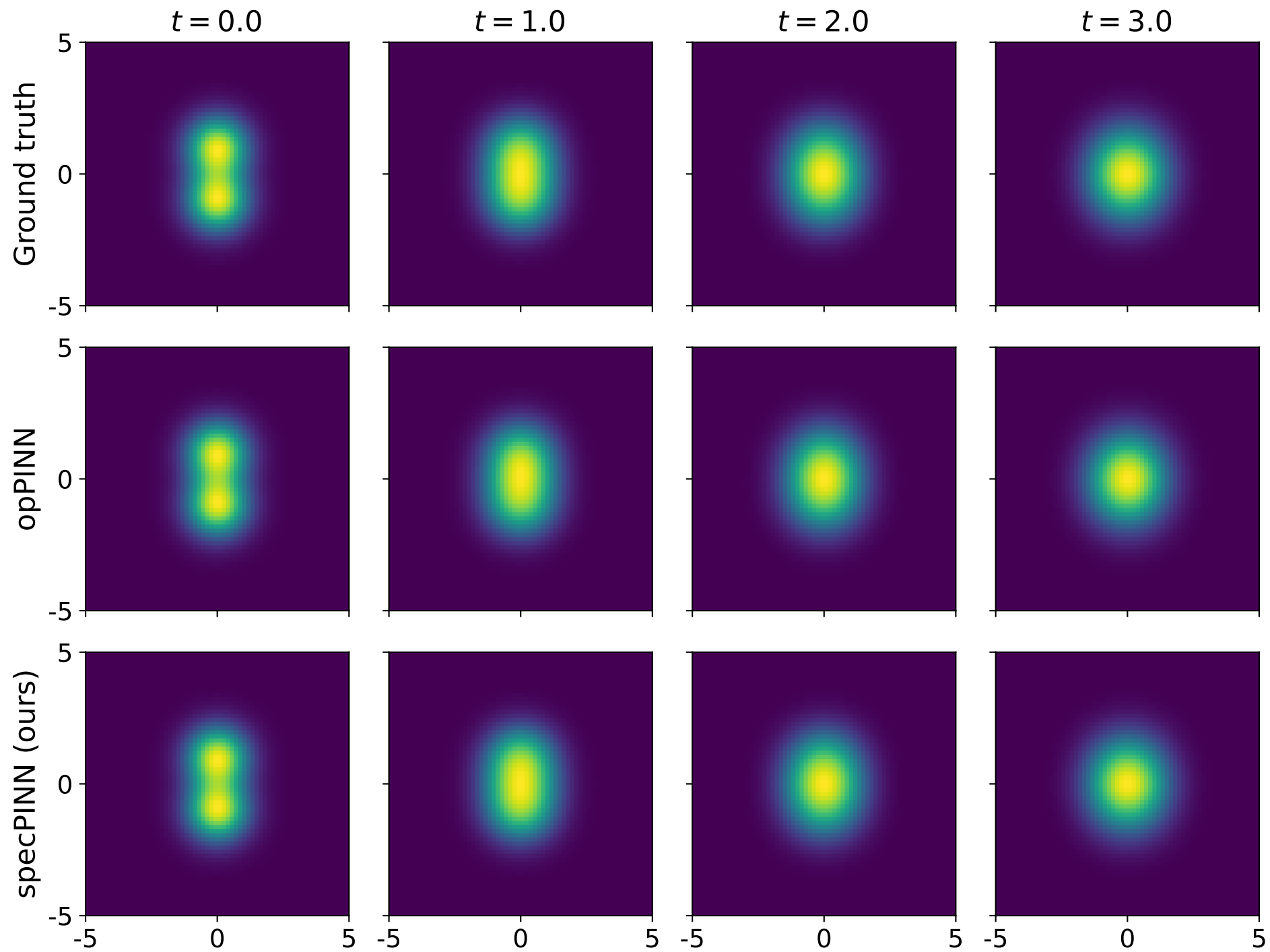
Sum of two Maxwellian distributions ( \gamma = -3.00 , \Lambda = 5.00 )
