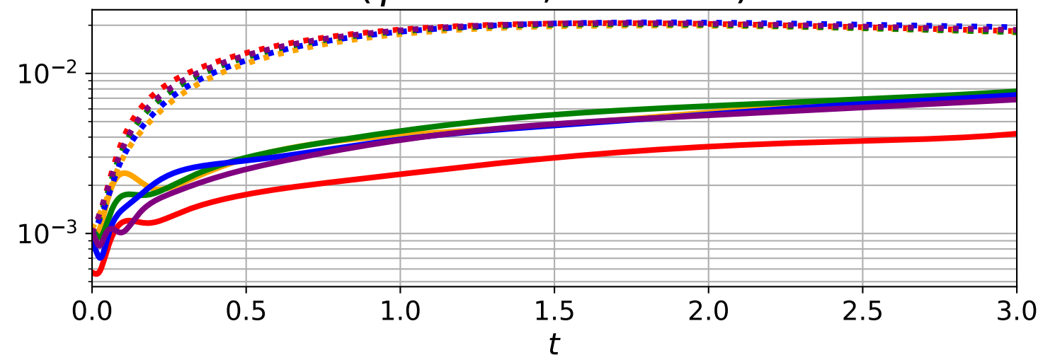
BKW solution ( \gamma = 0.00, \Lambda = 0.31 )
