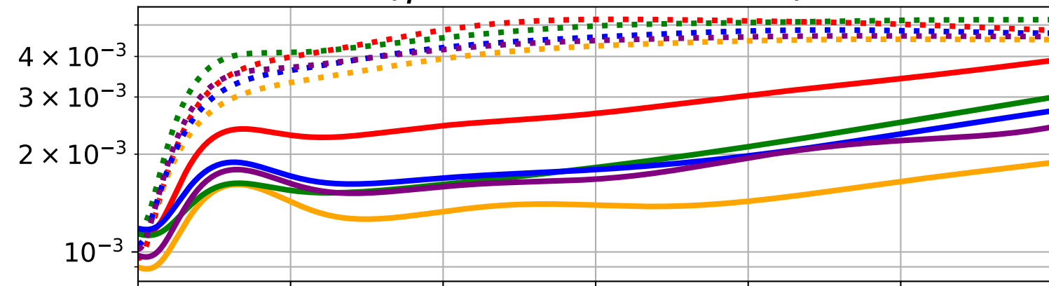
Sum of two Maxwellian distributions ( \gamma = 0.00, \Lambda = 0.31 )
