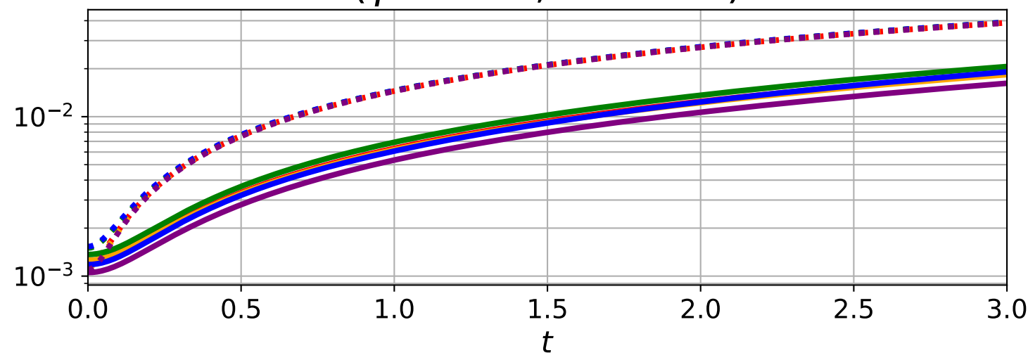
Maxwellian distribution ( \gamma = 0.00, \Lambda = 0.31 )
