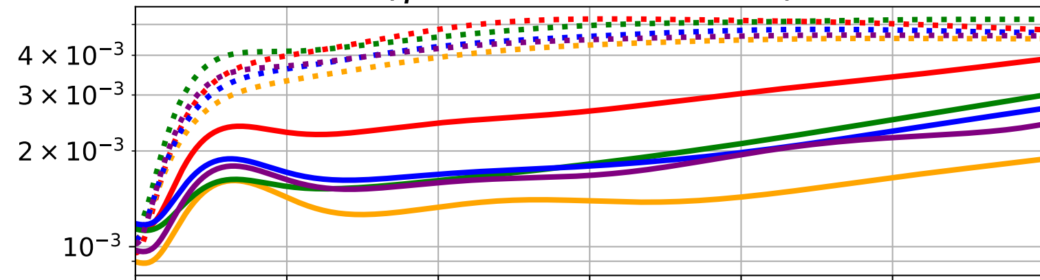
Sum of two Maxwellian distributions ( \gamma = 0.00, \Lambda = 0.31 )
