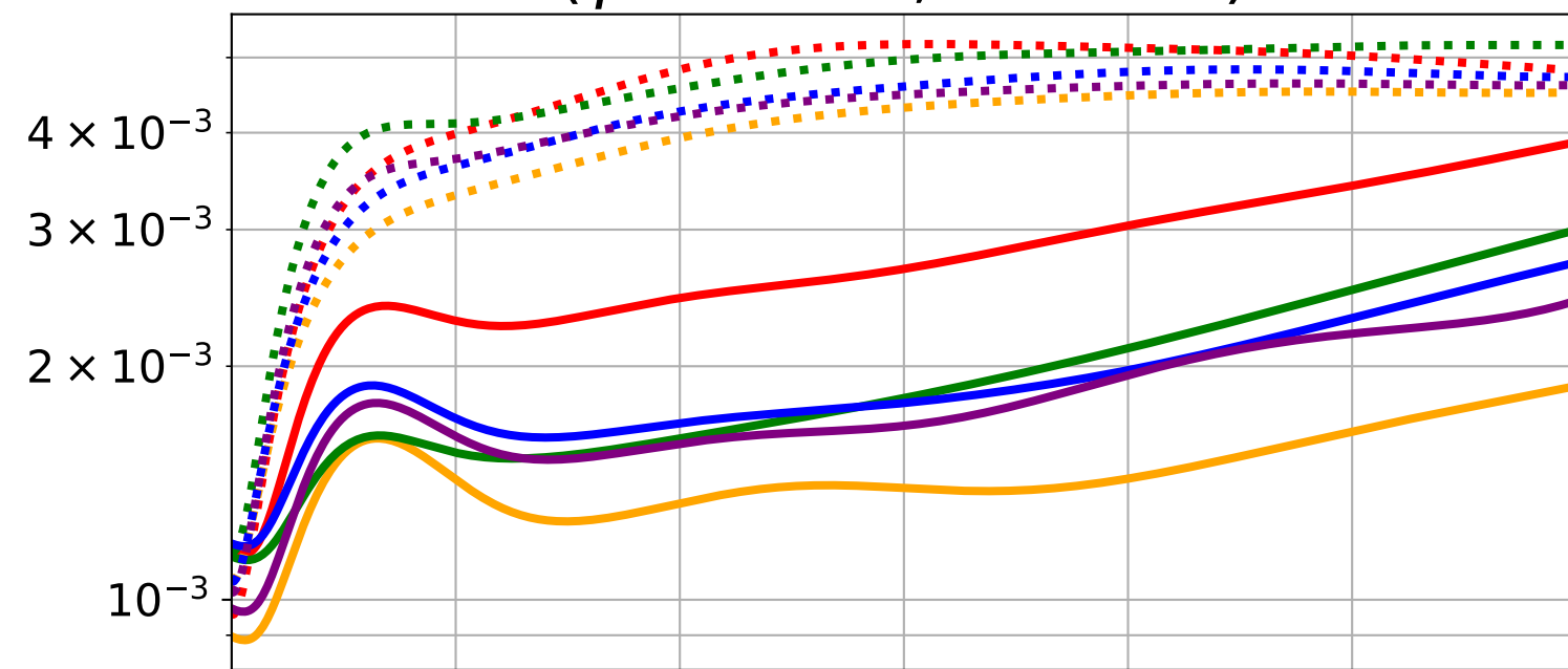
Sum of two Maxwellian distributions ( \gamma = 0.00, \Lambda = 0.31 )
