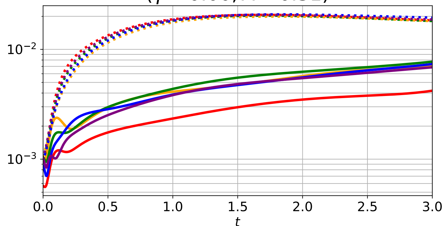
BKW solution ( \gamma = 0.00, \Lambda = 0.31 )
