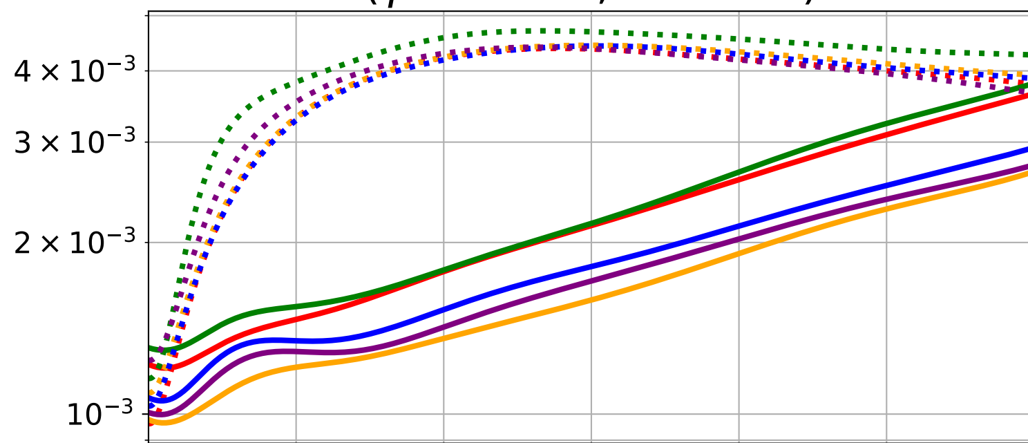
Maxwellian distribution ( \gamma = 0.00, \Lambda = 0.31 )
