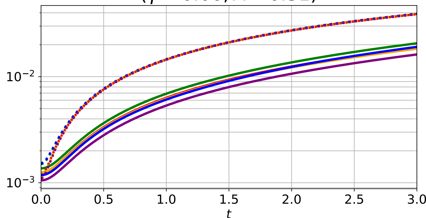
Maxwellian distribution ( \gamma = 0.00, \Lambda = 0.31 )
