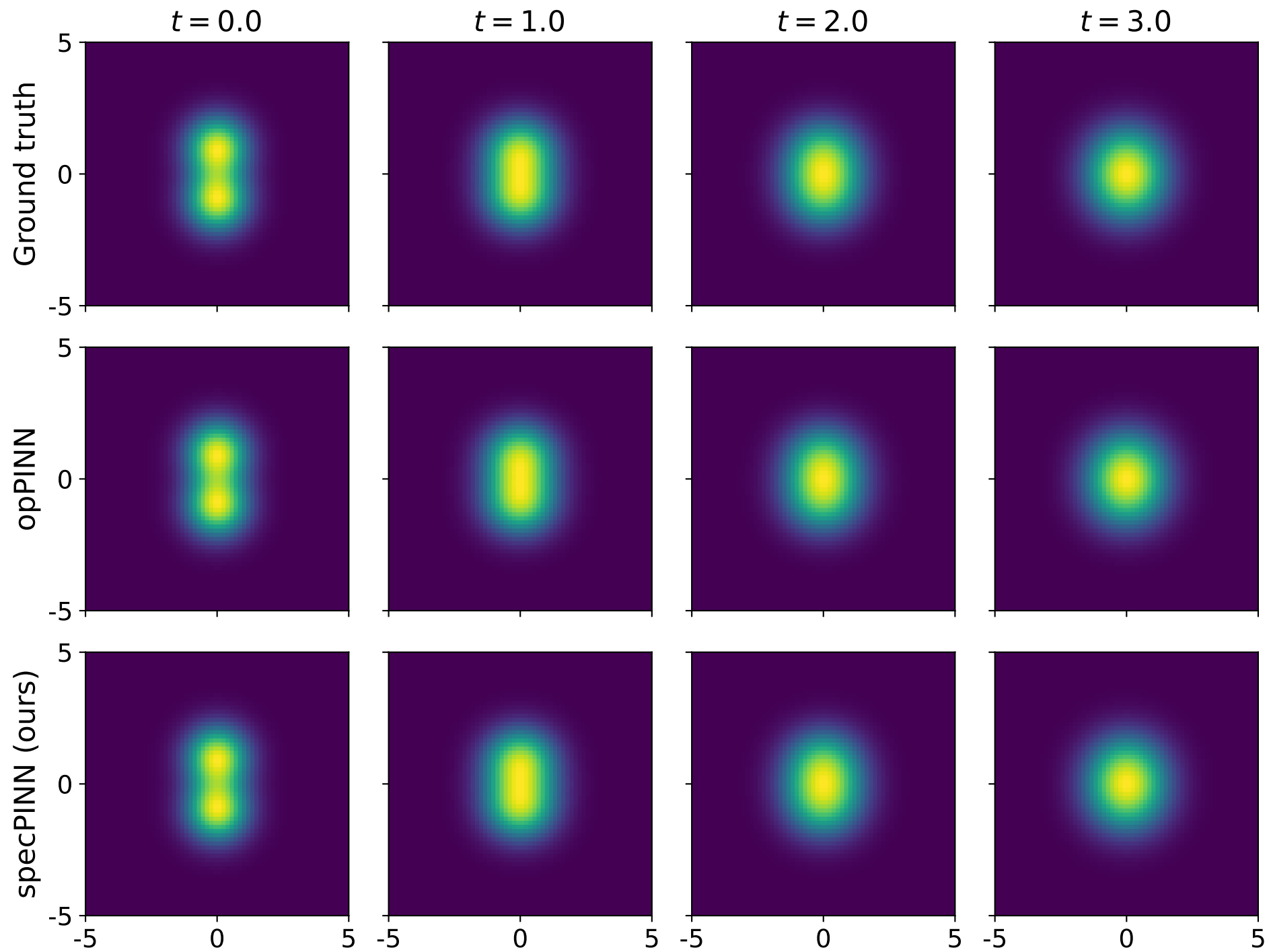
Sum of two Maxwellian distributions ( \gamma = -1.00 , \Lambda = 1.00 )
