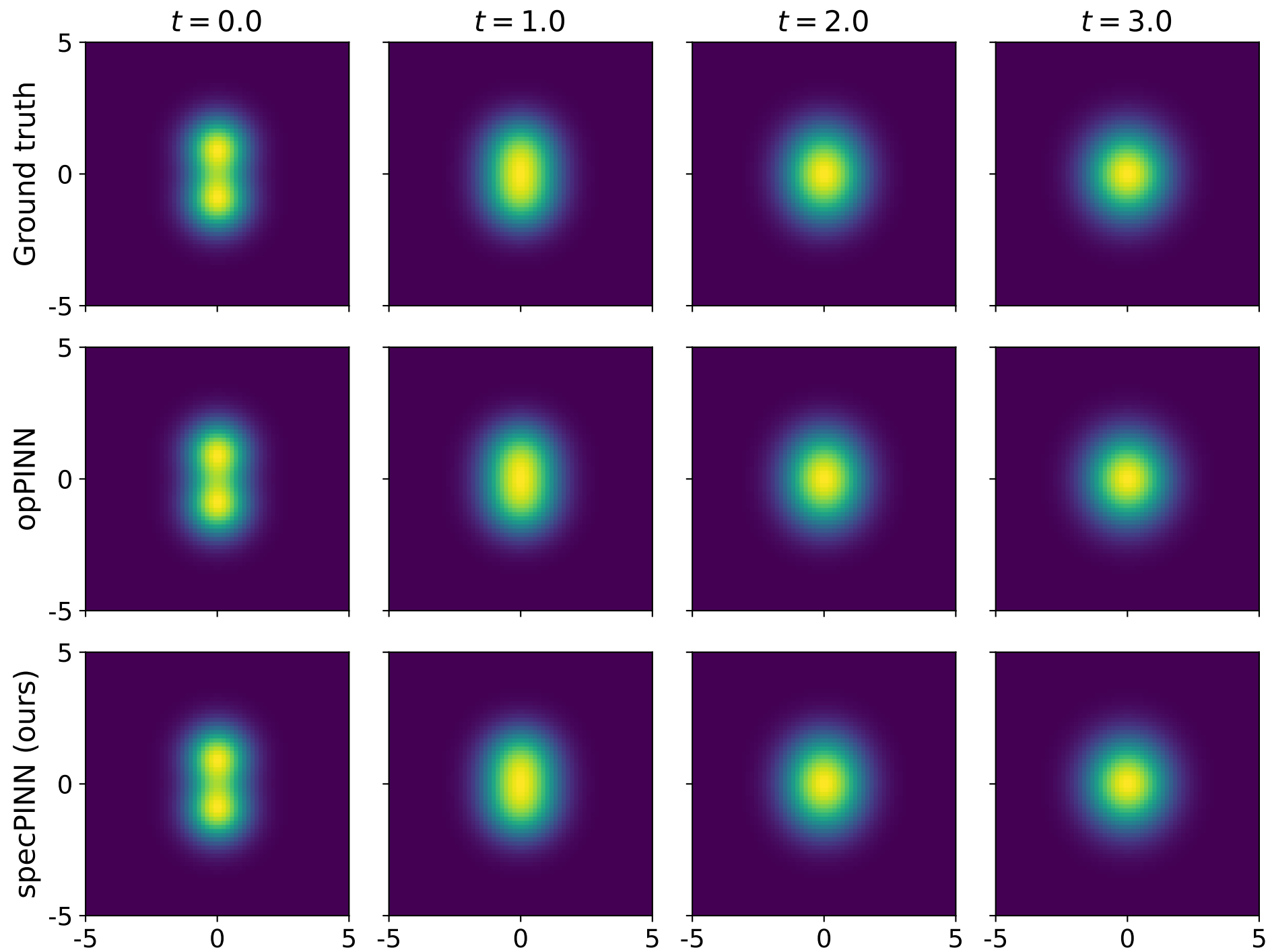
Sum of two Maxwellian distributions ( \gamma = -2.00 , \Lambda = 3.00 )
