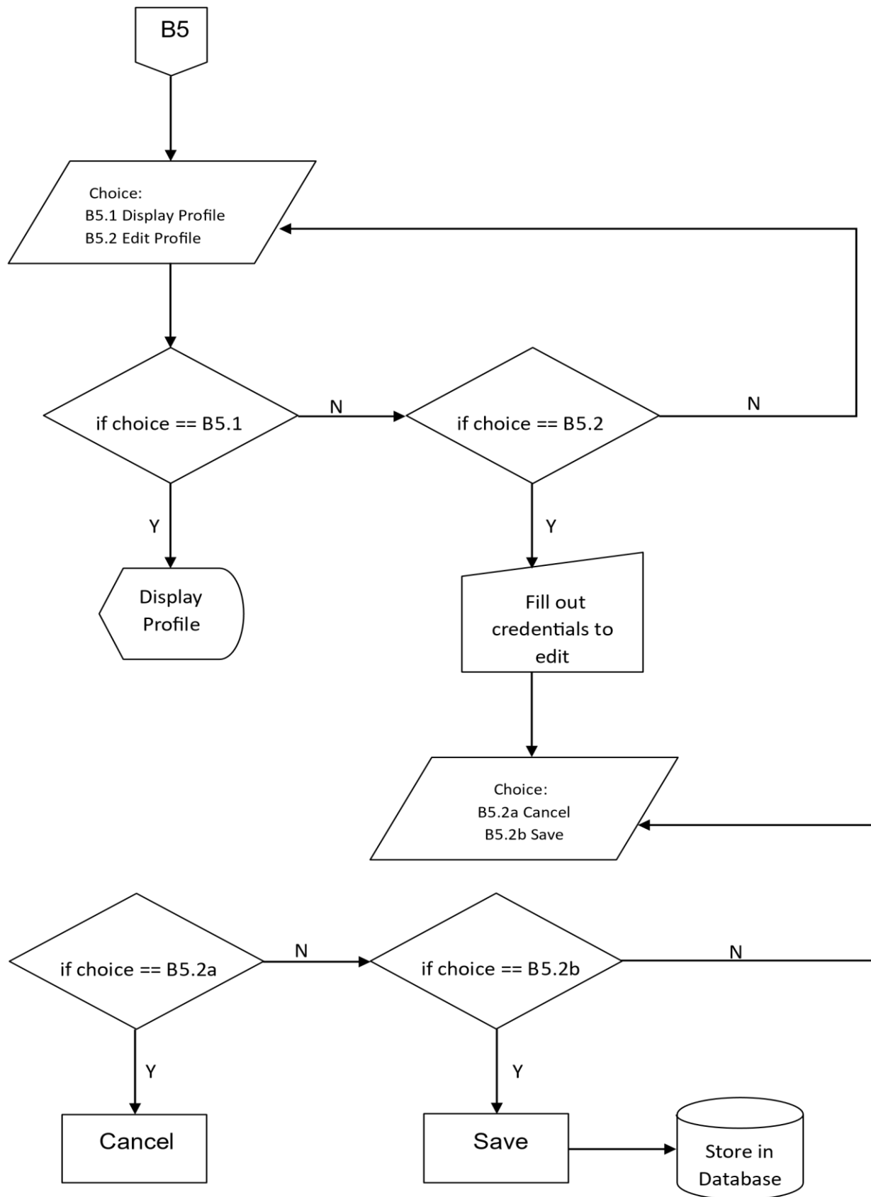
FIGURE 18. FACULTY PROFILE FLOWCHART
