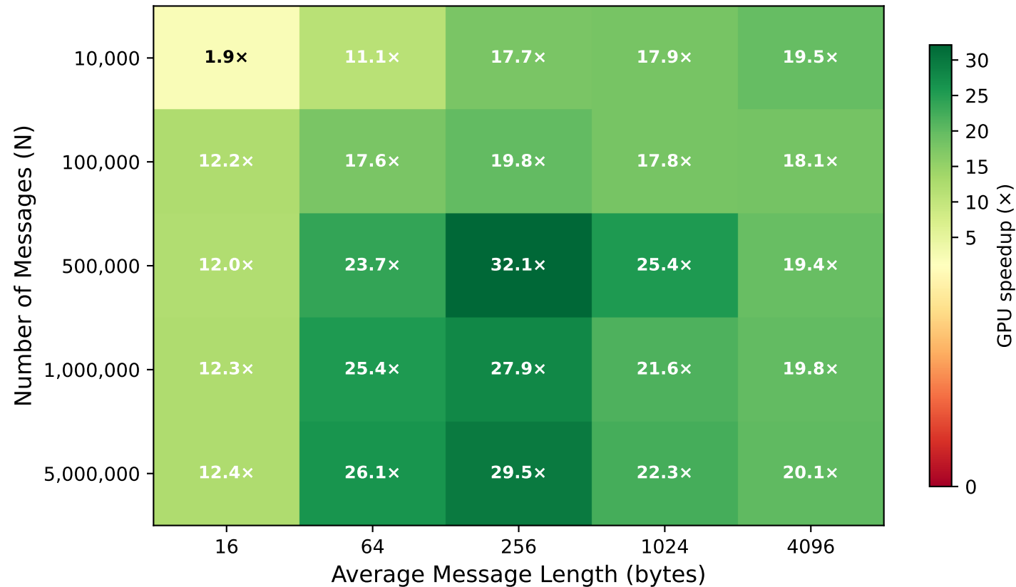
GPU End-to-End Speedup vs Single-Core CPU (SHA-256 Bulk Fingerprinting — B0 Baseline)
