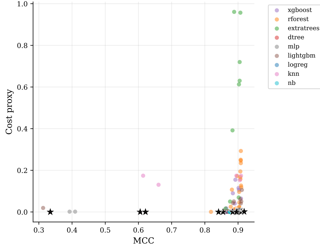
MCC vs. Cost (seed 0)
