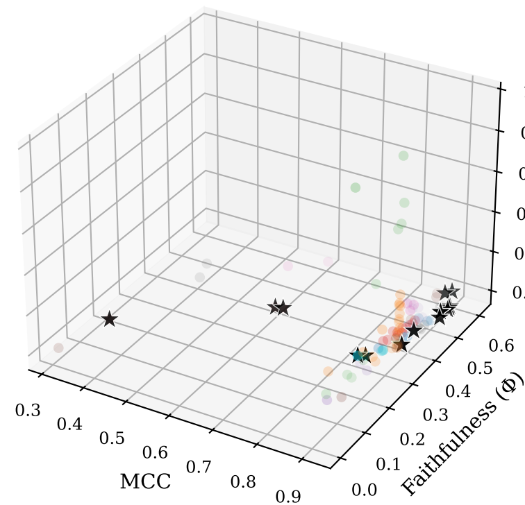
3D objective space — A1_dry_bean (seed 0)
