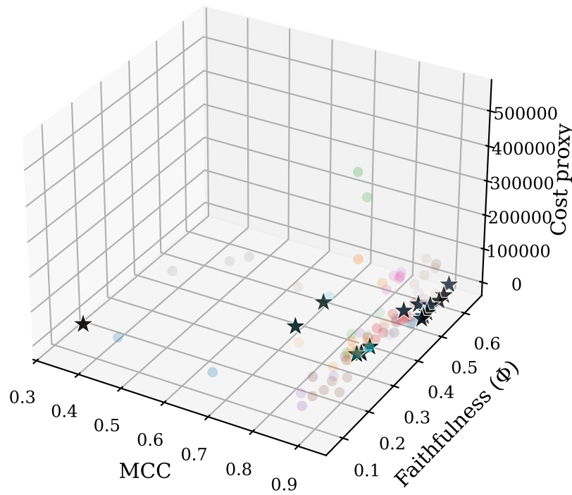
3D objective space — A1_dry_bean (seed 1)
