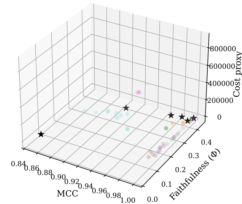
3D objective space — A2_mushroom (seed 2)
