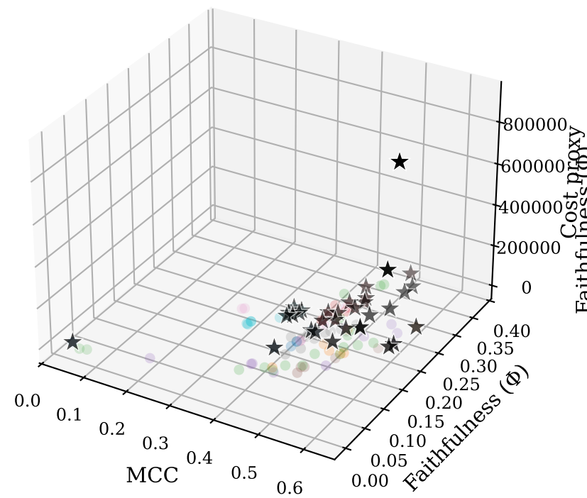
3D objective space — A3_wine_quality (seed 2)
