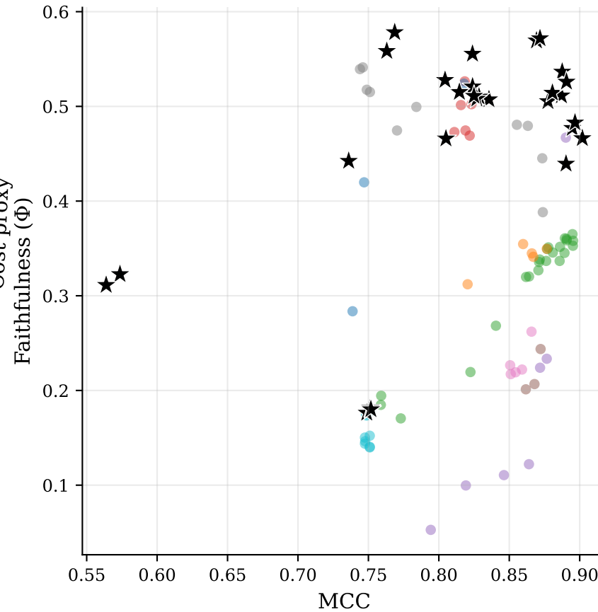
MCC vs. Faithfulness (seed 2)
