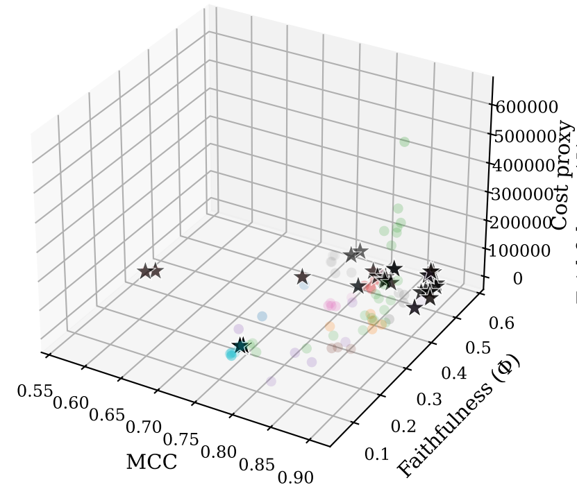
3D objective space — A4_landsat_satellite (seed 2)
