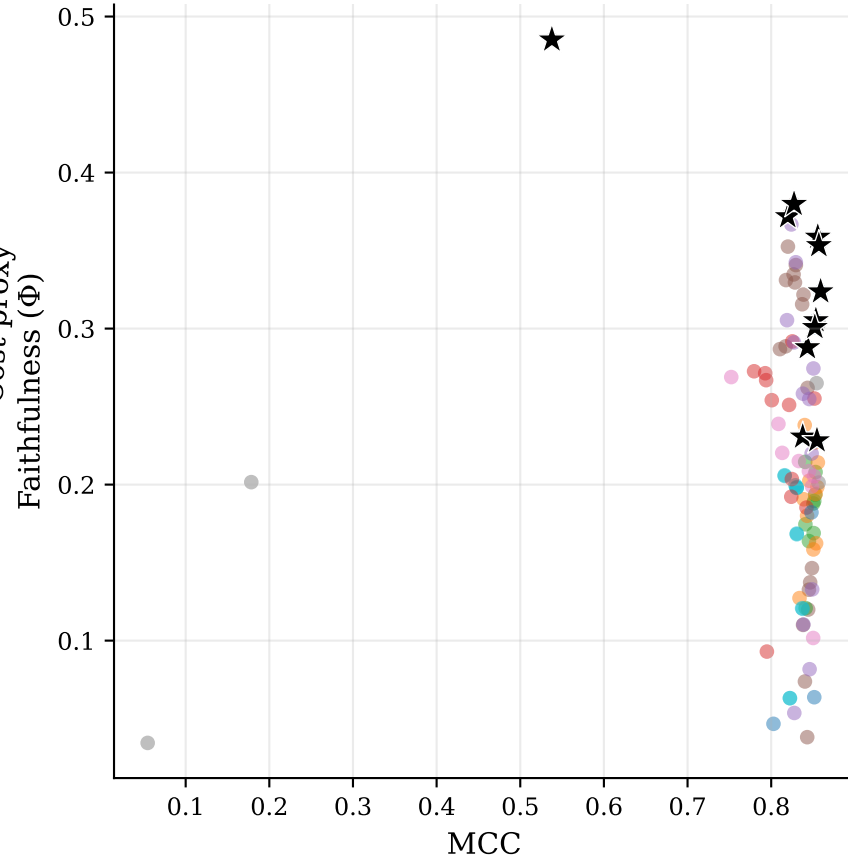
MCC vs. Faithfulness (seed 1)
