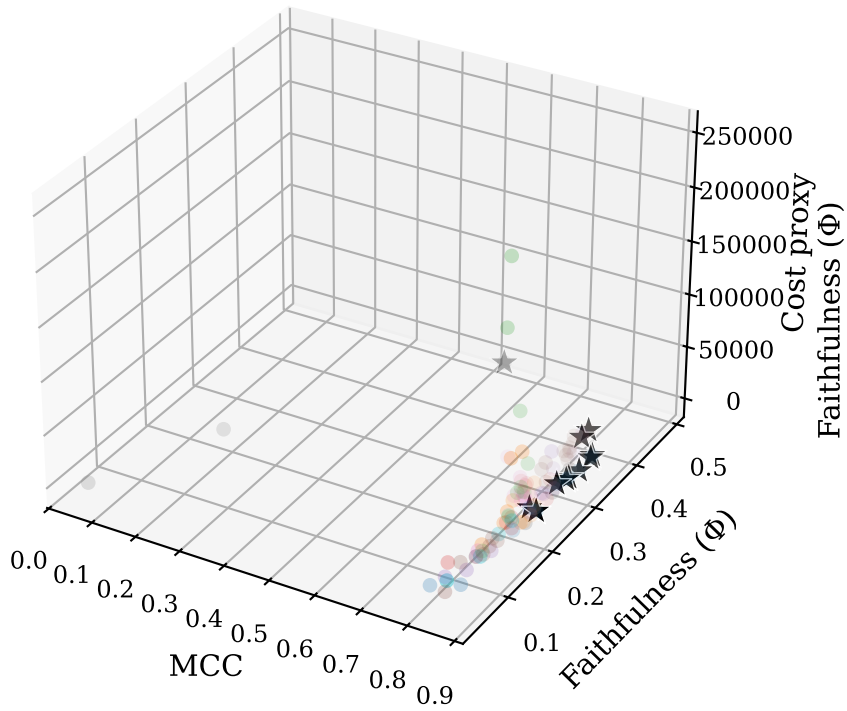
3D objective space — A5_rice (seed 1)
