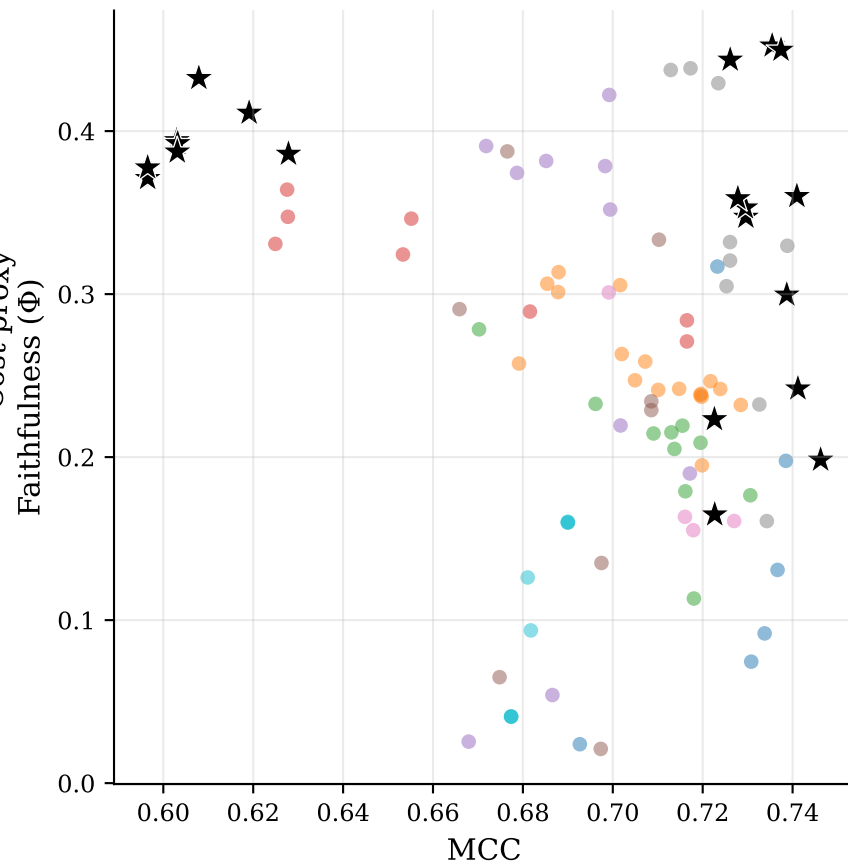
MCC vs. Faithfulness (seed 0)
