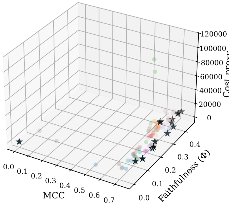
3D objective space — A6_raisin (seed 1)
