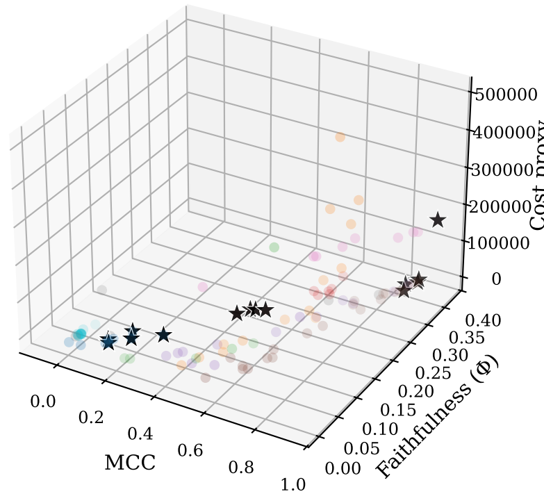
3D objective space — M1_eeg_eye_state (seed 1)
