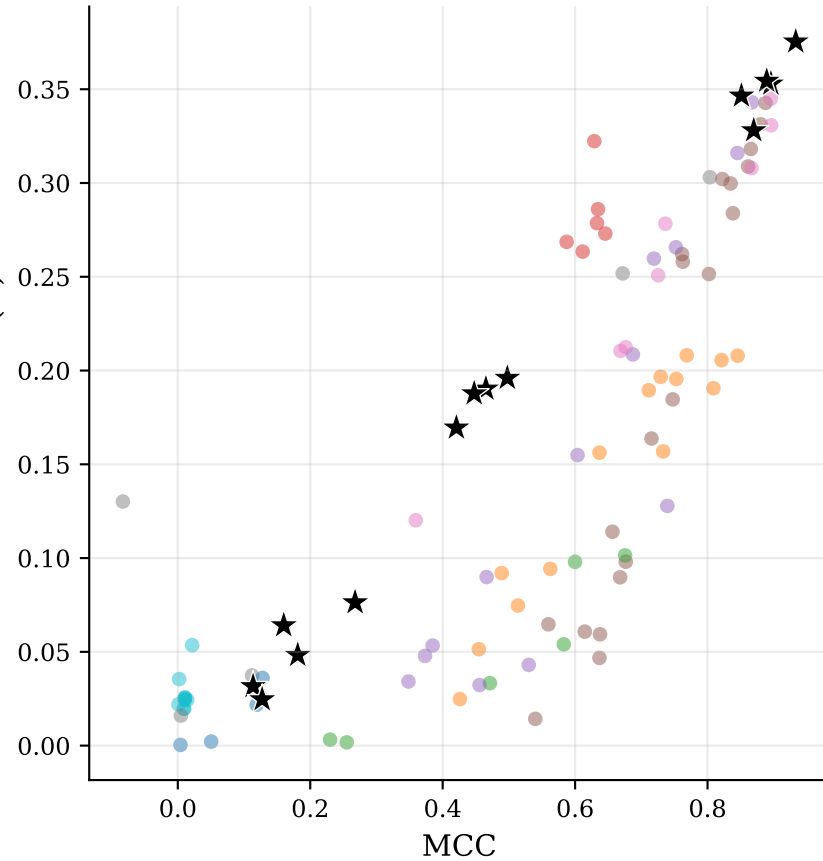
MCC vs. Faithfulness (seed 1)
