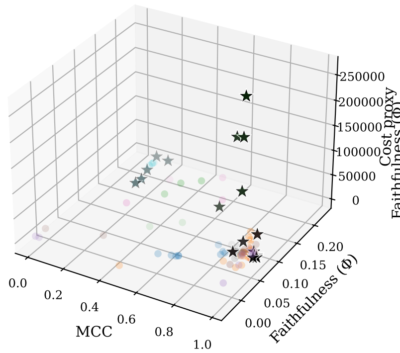
3D objective space — M2_thyroid_disease (seed 0)
