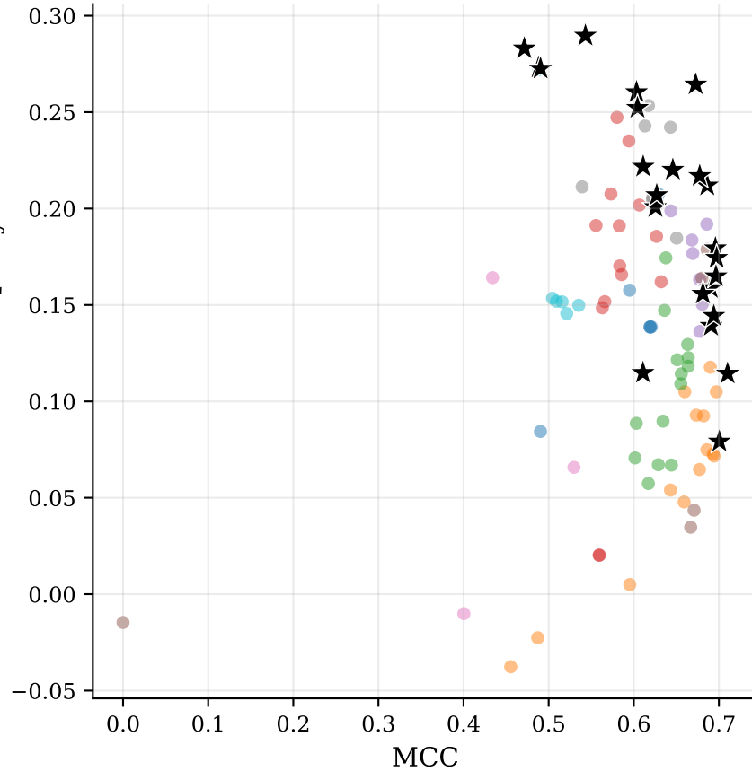
MCC vs. Faithfulness (seed 0)
