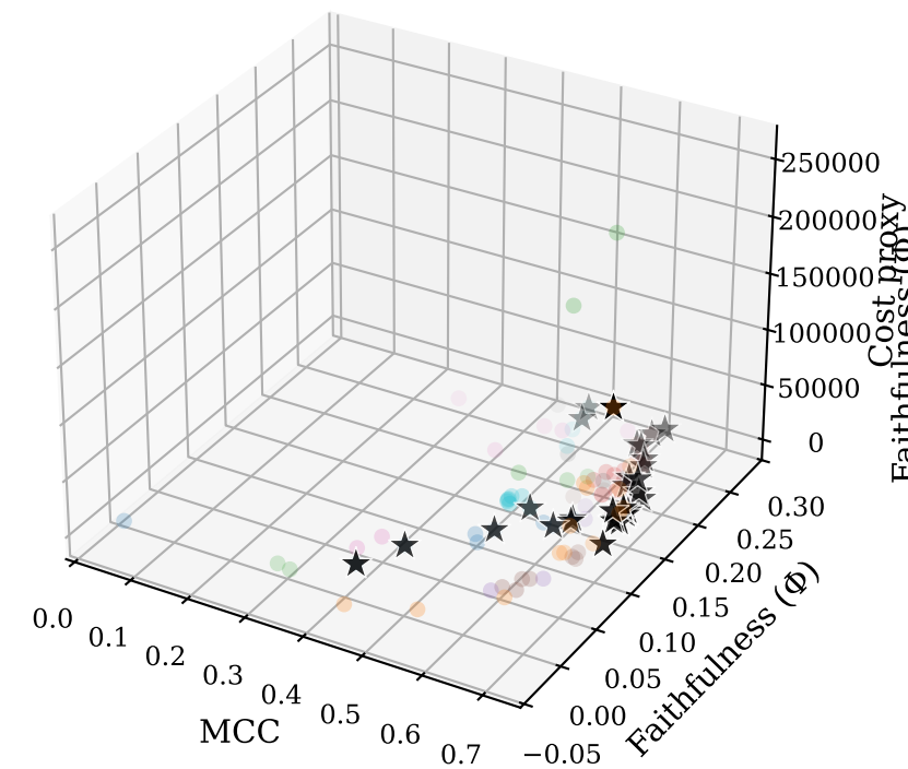
3D objective space — M3_aids_clinical_trials (seed 1)
