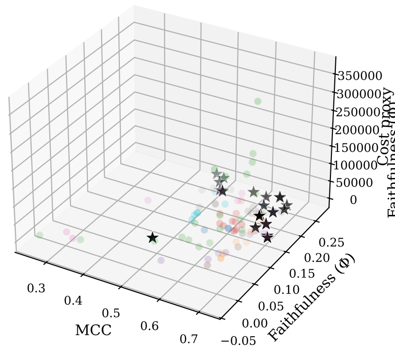
3D objective space — M3_aids_clinical_trials (seed 2)
