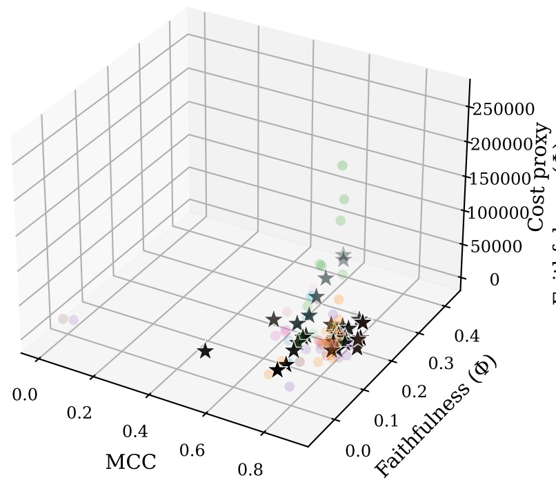
3D objective space — M4_cardiotocography (seed 0)
