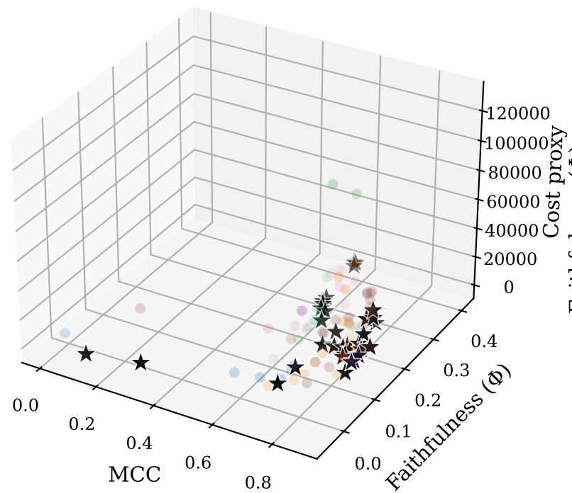
3D objective space — M4_cardiotocography (seed 1)
