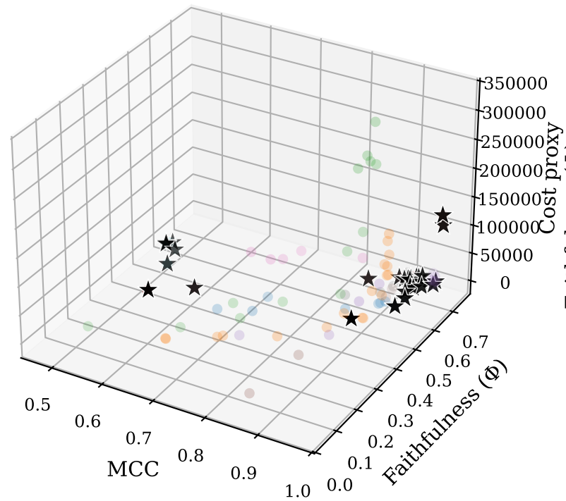
3D objective space — M5_obesity_levels (seed 0)
