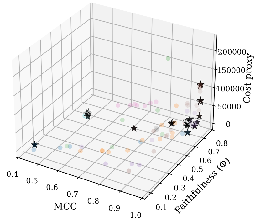
3D objective space — M5_obesity_levels (seed 1)
