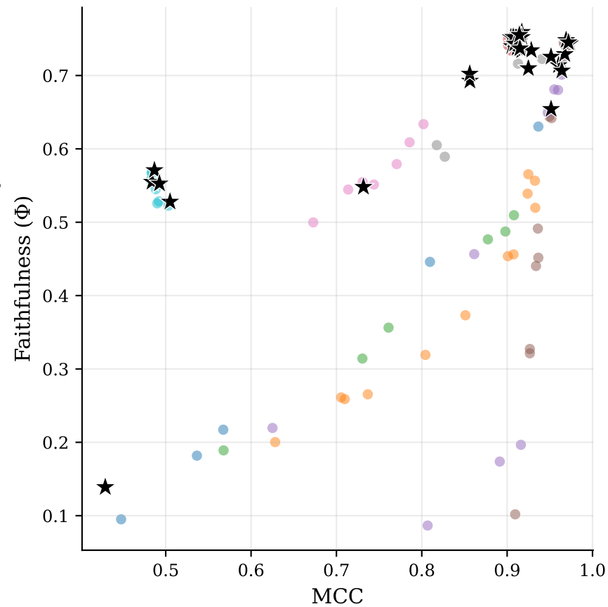
MCC vs. Faithfulness (seed 1)
