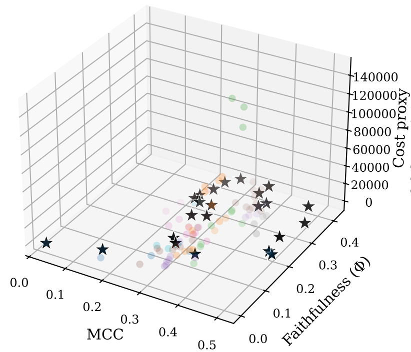
3D objective space — M6_diabetic_retinopathy (seed 1)
