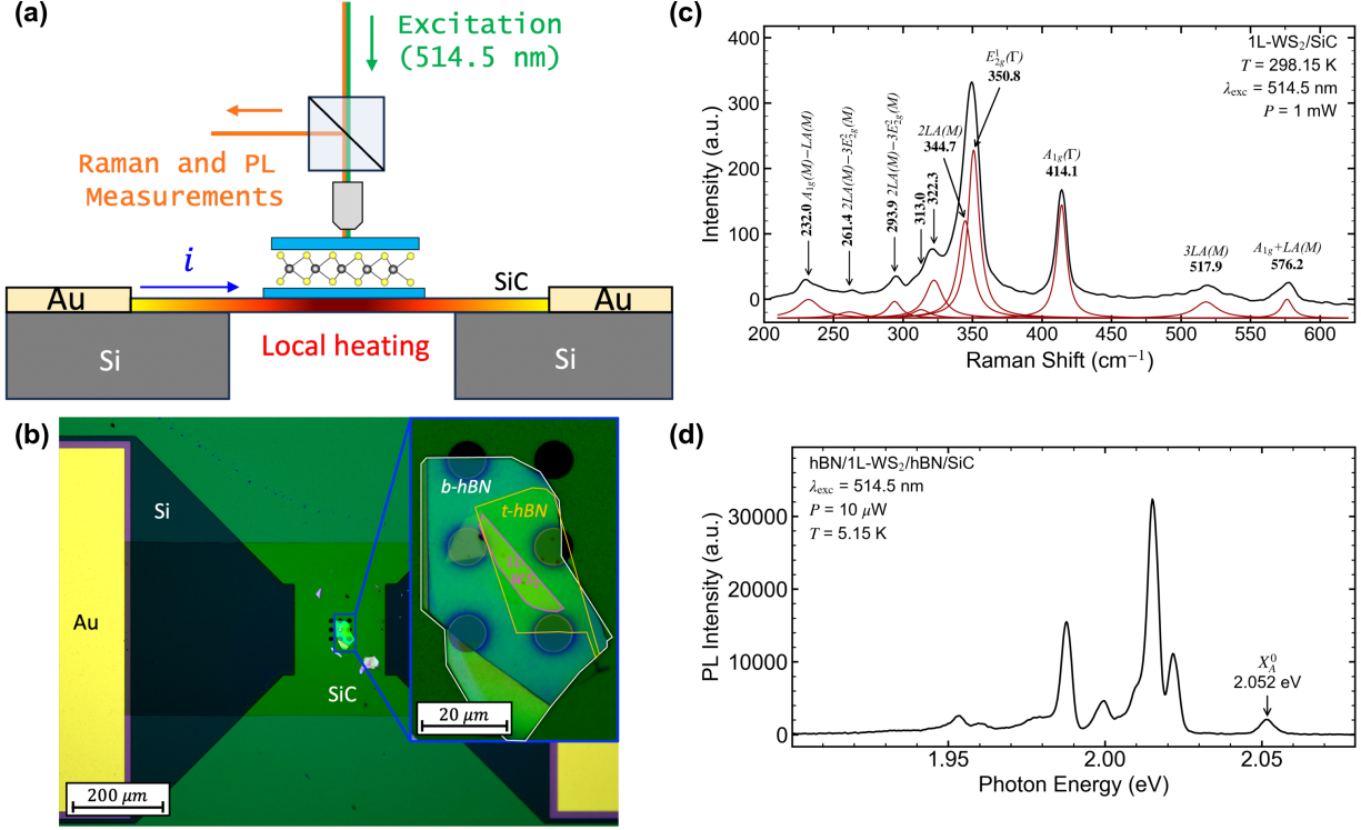
Figure 1: Experimental platform and reference spectra. (a) Schematic of the in-situ measurement platform: hBN/WS 2 /hBN heterostructure transferred onto the suspended SiC micro-membrane of the micro-heater chip, mounted inside a cryostat. (b) Optical image of the encapsulated WS 2 flake on the SiC membrane under white-light illumination. (c) Room-temperature Raman spectrum of non-encapsulated monolayer WS 2 ( \lambda_{\text{exc}} = 514.5 nm, P = 1 mW), including Lorentzian peak fits for the E_{2g}^1(\Gamma) , 2LA(M) , A_{1g}(\Gamma) , and higher-order combination modes. High-power illumination induces photodoping in the absence of hBN encapsulation, precluding PL measurements on this sample. (d) PL spectrum of hBN-encapsulated WS 2 at 5 K, showing the neutral exciton X_A^0 , trion, and dark-exciton-related features ( \lambda_{\text{ex}} = 514.5 nm, P = 10 \mu W).
