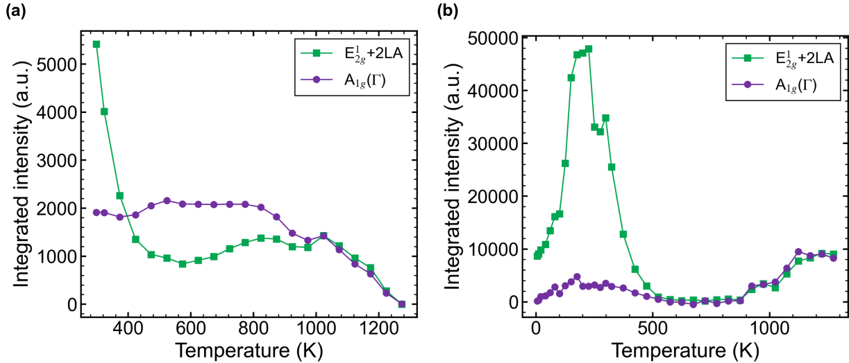
Figure S7: Integrated Raman intensity of the \text{E}_{2g}^1 + 2\text{LA} band (green squares) and the \text{A}_{1g} mode (purple circles) versus temperature for (a) the non-encapsulated and (b) the hBN-encapsulated sample. Intensities are in arbitrary units and are not comparable between the two samples.
