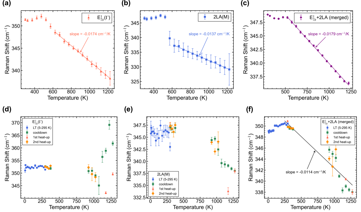
Figure S1: Individual versus merged-peak fitting of the E_{2g}^1 + 2LA doublet. Top row: non-encapsulated sample – (a) E_{2g}^1 individual fit, (b) 2LA individual fit, (c) merged-peak fit ( T \geq 500 \text{ K} linear fit shown). Bottom row: hBN-encapsulated sample – (d) E_{2g}^1 individual fit, (e) 2LA individual fit, both showing instability above \sim 900 \text{ K} , (f) merged-peak fit, pooled linear fit over T \geq 250 \text{ K} across all four measurement stages.
