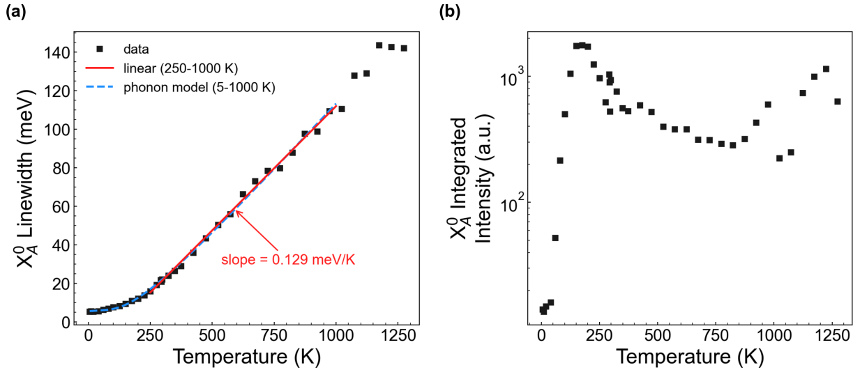
Figure S5: Temperature dependence of the PL linewidth and intensity. (a) Total Voigt FWHM \Gamma_V of the X_A^0 emission versus temperature. Blue dashed line: phonon-scattering model fitted over 5–1000 K; red line: linear fit over 250–1000 K. (b) Integrated X_A^0 PL intensity versus temperature, showing the thermally activated rise from the dark-exciton ground state below \sim 175 K and the subsequent thermal quenching at higher temperature.
