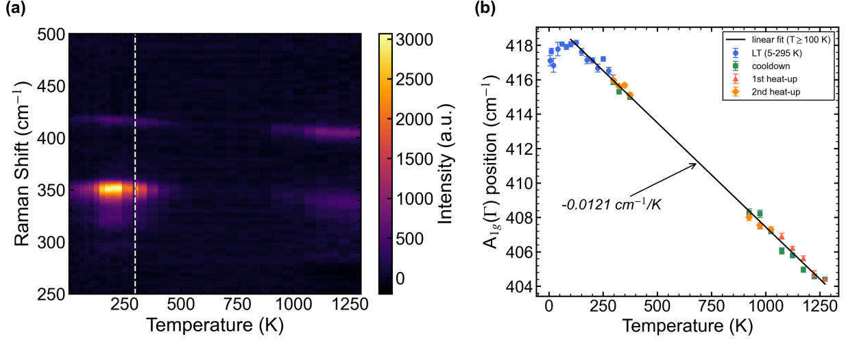
Figure S2: Temperature-dependent Raman response of the hBN-encapsulated WS 2 monolayer. (a) Two-dimensional map of Raman intensity versus temperature (5–1273 K) and Raman shift; the dashed line marks the boundary between the cryostat (5 K–RT) and micro-heater (RT–1273 K) stages. (b) A 1g peak position versus temperature for each measurement stage. The solid line is a linear fit to this sample over T \geq 100 K ( -0.0121 \text{ cm}^{-1}/\text{K} ), as used in the main text; cooldown and heat-up data scatter around the same line.
