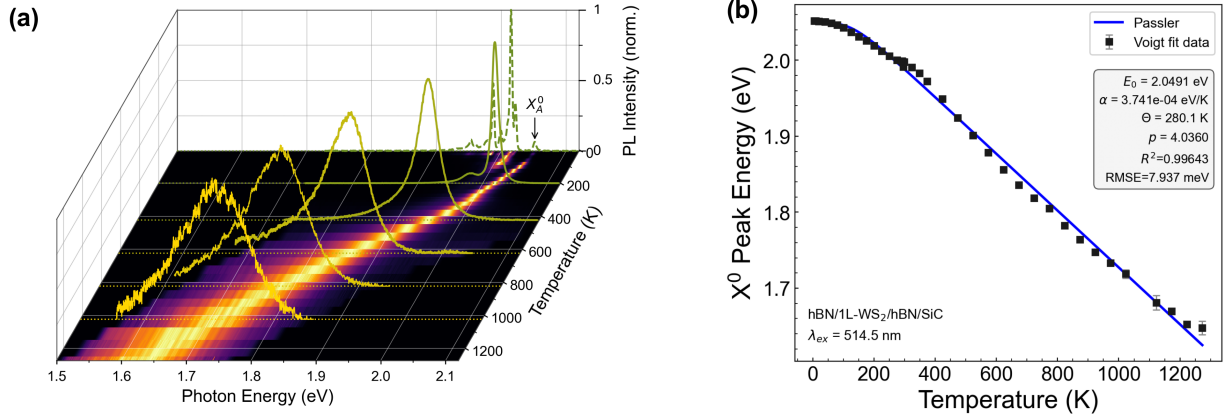
Figure 3: Photoluminescence thermal indicator in hBN-encapsulated monolayer WS 2 . (a) Waterfall plot of representative PL spectra (5 K to 1023 K) as a function of photon energy, normalized to the peak intensity at each temperature, overlaid on the full temperature-dependent intensity map. The X_A^0 neutral-exciton peak, visible at low temperature, redshifts and broadens continuously with increasing temperature. (b) Neutral-exciton peak energy E_0 extracted from Voigt fits (black squares, with error bars) and the Pässler model fit (blue line), Eq. (2), with best-fit parameters and fit quality annotated.
