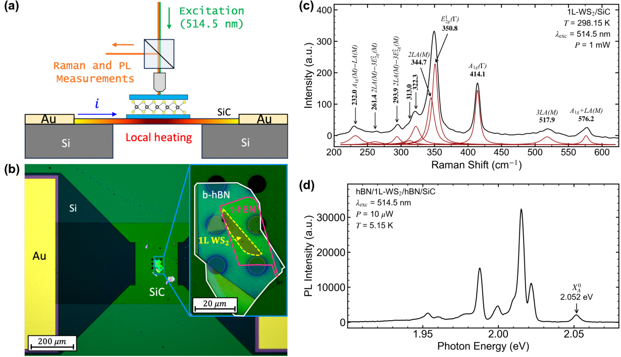
Figure 1: Experimental platform and reference spectra. (a) Schematic of the in-situ measurement platform: hBN/WS 2 /hBN heterostructure transferred onto the suspended SiC micro-membrane of the micro-heater chip, mounted inside a cryostat. (b) Optical image of the encapsulated WS 2 flake on the SiC membrane under white-light illumination. (c) Room-temperature Raman spectrum of non-encapsulated monolayer WS 2 ( \lambda_{\text{exc}} = 514.5 nm, P = 1 mW), including Lorentzian peak fits for the E_{2g}^1(\Gamma) , 2LA(M) , A_{1g}(\Gamma) , and higher-order combination modes. High-power illumination induces photodoping in the absence of hBN encapsulation, precluding PL measurements on this sample. (d) PL spectrum of hBN-encapsulated WS 2 at 5 K, showing the neutral exciton X_A^0 , trion, and dark-exciton-related features ( \lambda_{\text{ex}} = 514.5 nm, P = 10 μW).
