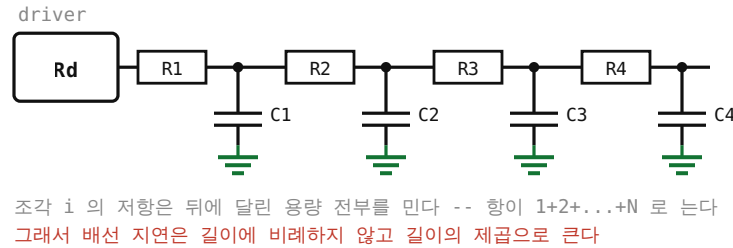
그림 2. A wire cut into four RC sections. Section 1's resistance pushes the capacitance of sections 1–4; section 4's pushes only its own.
