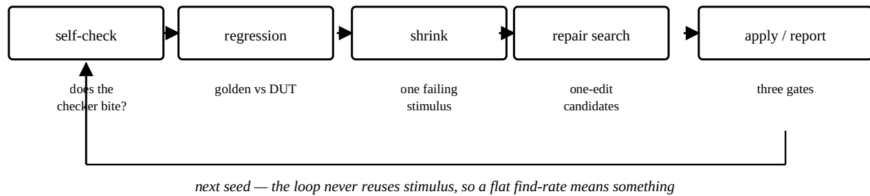
Figure 62. One iteration of the loop. The first box is the one most regression systems lack, and it is the reason the rest can be believed.
