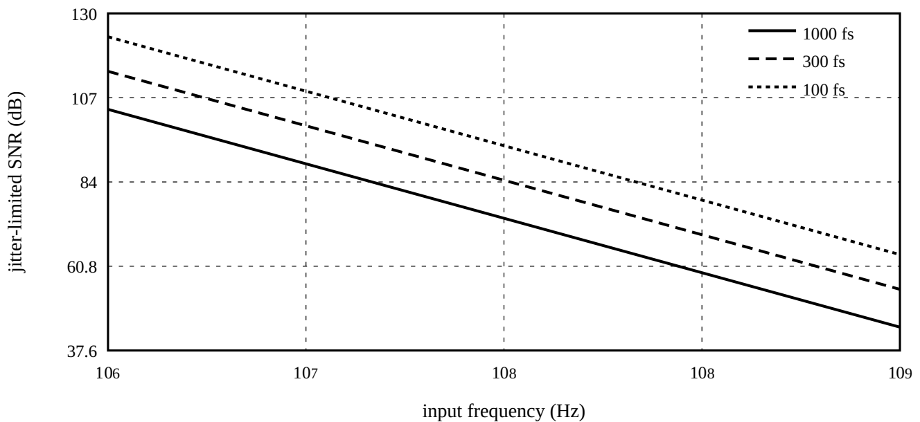
Figure 35. The jitter wall. Every curve falls 20 dB per decade of input frequency; the only way up is a better clock.
