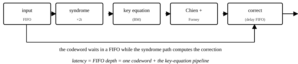
Figure 56. The decoder architecture. The delay FIFO is the block’s dominant memory and the reason latency is quoted in code-words.
