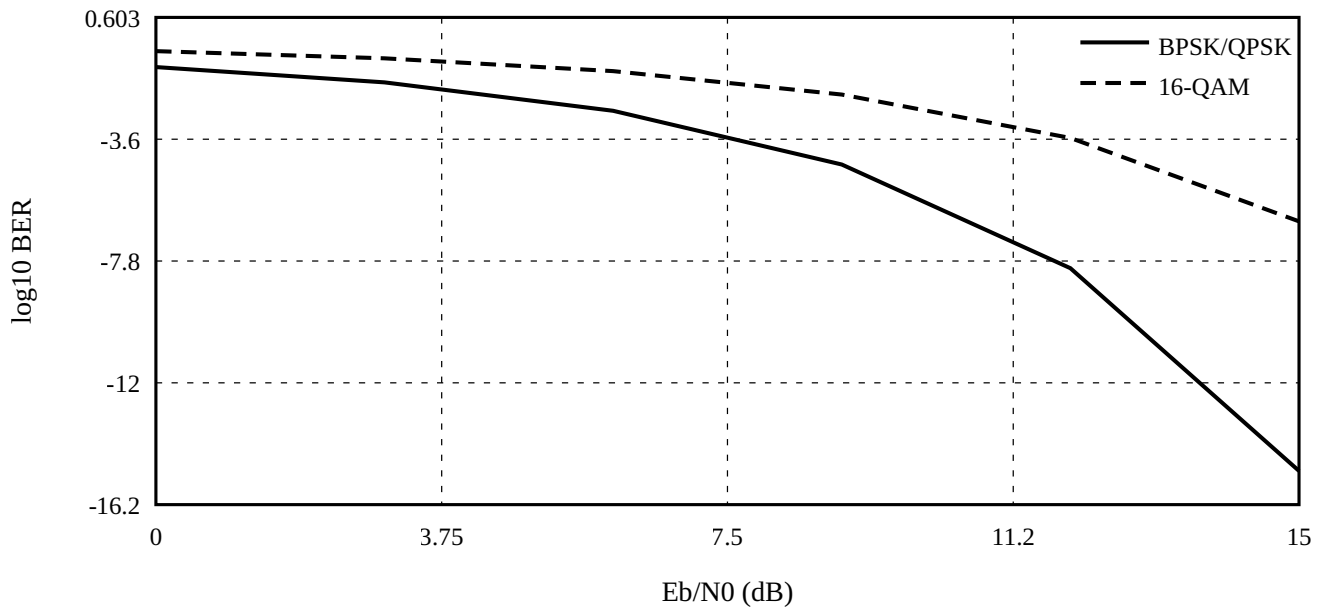
Figure 42. The waterfall curves. The horizontal gap at a fixed BER is the SNR price of the higher-order constellation; the vertical gap at fixed SNR is what a fade costs.
